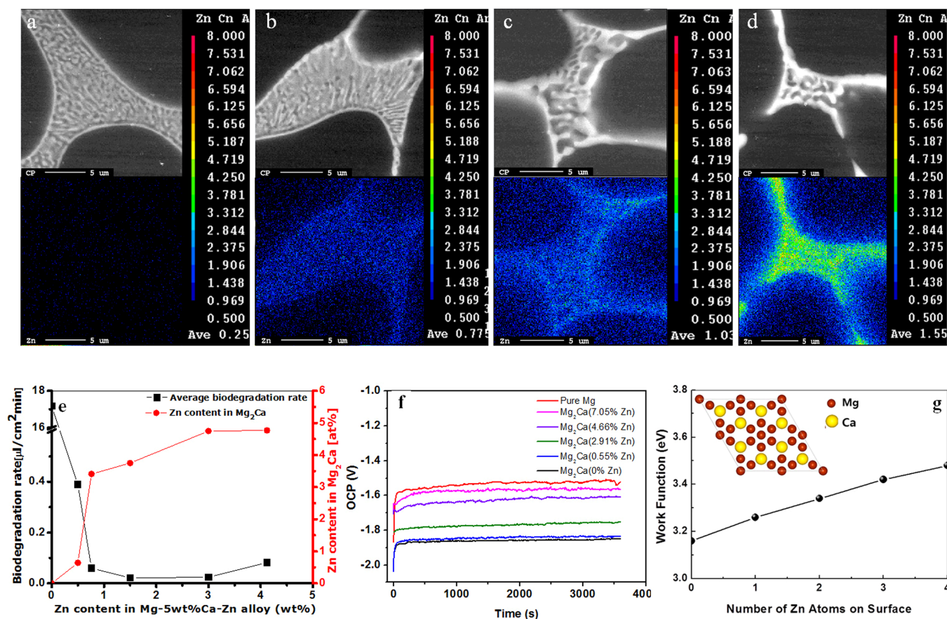
Figure 2 | (a–d). SEM and the corresponding WDS images showing the distribution of dissolved Zn in Mg-5 wt%Ca- x wt%Zn alloys ( x = 0, 0.5, 1.0 , and 1.5 from the left). (e). Relationship between the biodegradation rate of Mg-Ca-Zn alloys and the Zn concentration inside Mg 2 Ca obtained from WDS analysis. (f). Measurement of the open-circuit potential (OCP) of the immersed Mg 2 Ca alloys with various Zn concentrations. (g). Variation of the work function with Zn contents in the (0001) surface of Mg 2 Ca (Inset. Atomic configuration of the (0001) surface where red spheres represents Mg atom and gold spheres represent Ca atom).
