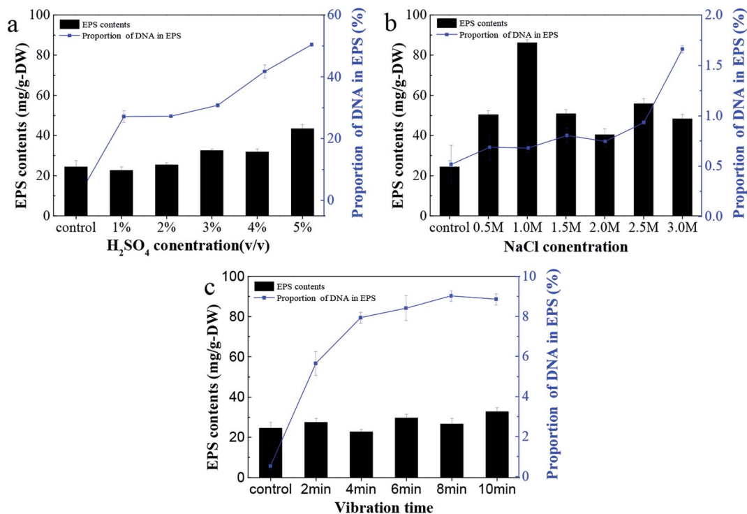
Fig. 2 The efficiencies of EPS extraction from C. pauculus 1490 and relevant proportions of DNA in EPS from the three methods: (a) the sulfuric acid method with varied H_2SO_4 concentrations, (b) the sodium chloride method with varied NaCl concentrations, and (c) the vibration method with varied vibration times by glass beads.
