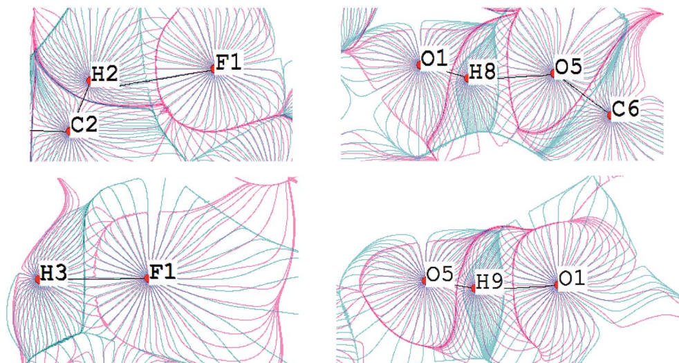
Fig. 10 Superposition of gradient fields of the electrostatic potential (pink) and the electron density (blue) for the TISQER crystal. The bond paths are given by black lines. The nuclei positions are given by red circles. For atomic labels see Fig. S6.†
