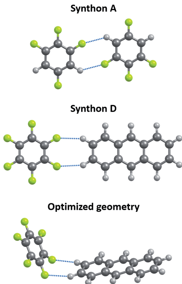
Fig. 1 C–H⋯F–C synthons referred to in this study. C–H⋯F dimer motif in the o -C 6 H 2 F 4 crystal (synthon A) and C–H⋯F–C dimer motif in the cocrystal of C 6 F 6 and anthracene (synthon D). Spatial orientation of molecules in the C 6 F 6 – anthracene dimer, obtained as a result of optimization at the PBE/6-31(F+)G** approximation (lower panel). H⋯F interactions are denoted by dotted lines.
