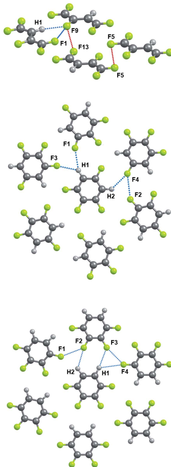
Fig. 3 Fragments of crystalline C 4 HF 5 (upper panel), m -C 6 H 2 F 4 (middle panel) and o -C 6 H 2 F 4 (lower panel). The C–H⋯F–C and C–F⋯F–C interactions are denoted by dotted lines. Two types of C–F⋯F–C contacts occur in C 4 HF 5 crystal, namely, intra- and interlayer ones. The latter are shown with red dotted lines.
