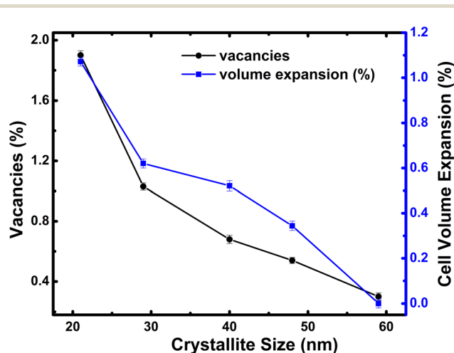
Fig. 1 Variation of oxygen vacancy concentration and unit cell volume for all the crystallite sizes of h-FP.
