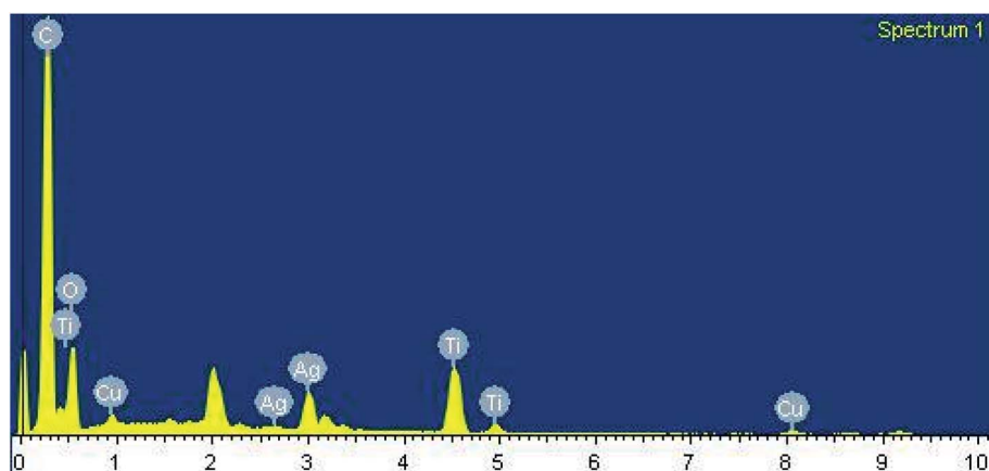
Fig. 4 EDX spectrum of Cu@Ag-TiO 2 -NGO.
