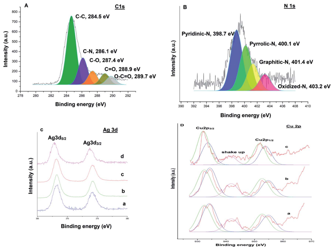
Fig. 9 (A) XPS spectrum of C 1s; (B) XPS spectrum of N 1s; (C) XPS spectra depicting comparison of Ag 3d region, (a) monometallic Ag@TiO 2 -NGO; (b) bimetallic Cu@Ag-TiO 2 -NGO; (c) re-used Cu@Ag-TiO 2 -NGO in case of oxidation; (d) re-used Cu@Ag-TiO 2 -NGO in case of C-N coupling. (D) XPS spectra depicting comparison of Cu 2p region, (a) bimetallic Cu@Ag-TiO 2 -NGO; (b) re-used Cu@Ag-TiO 2 -NGO in case of oxidation; (c) re-used Cu@Ag-TiO 2 -NGO in case of C-N coupling.
