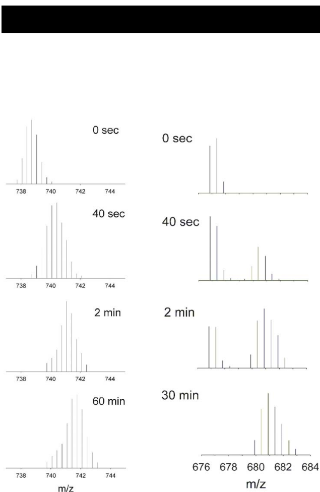
Figure 4 Example of HDX detected by mass spectra. m/z isotopic envelopes for EX2 (A) and EX1 (B) limit of exchange. Data obtained for a region that is situated within the subunit interface in \phi 8 P4 hexamer [114].
