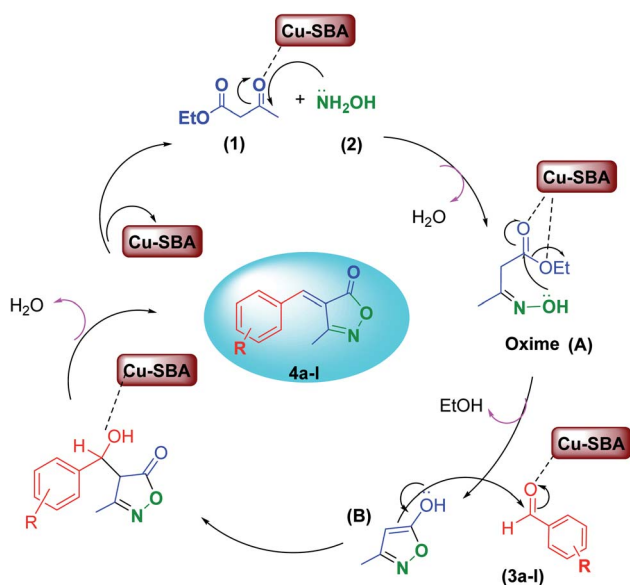
Scheme 3 Proposed catalytic cycle for the synthesis of 4-aryl-methylene isoxazole-5(4H)-ones using Cu/TCH-pr@SBA-15.
