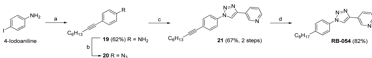
Scheme 7. Synthesis of RB-054 from 4-Iodoaniline a
