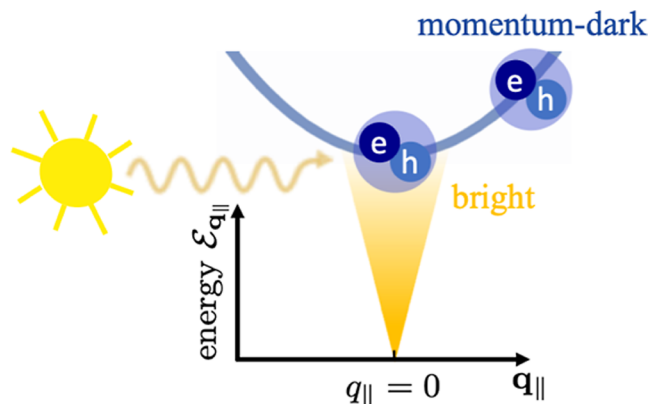
Figure 2. Parabolic exciton dispersion \mathcal{E}_{q_{\parallel}} over center-of-mass momentum q_{\parallel} . A bright and a momentum-dark exciton are indicated exemplarily. The schematic “sun” represents a radiative excitation from the far-field.
