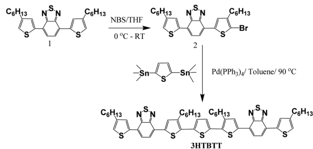
Scheme 1 Synthesis route for 3HTBTT small molecule.
