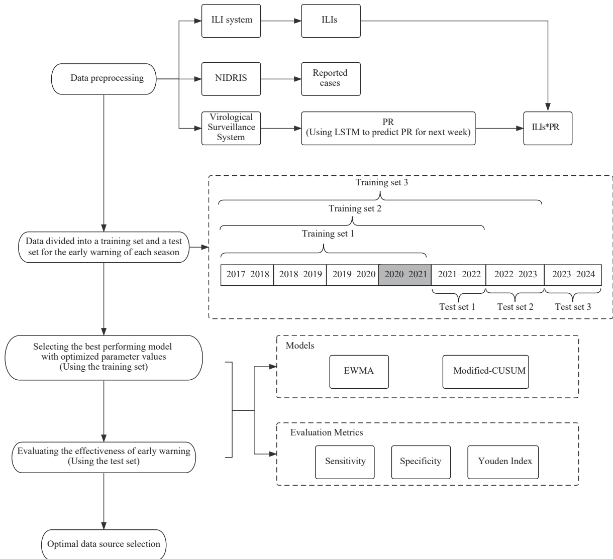
SUPPLEMENTARY FIGURE S1. Flowchart of early warning model construction and performance evaluation.
