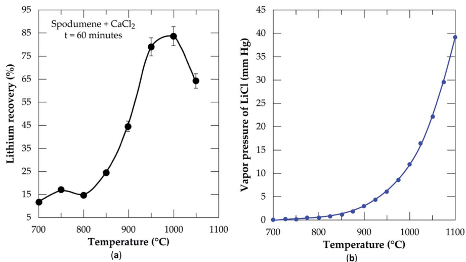
Fig. 6 (a) Percent lithium recovery versus temperature at \text{CaCl}_2/\text{spodumene} molar ratio of 2.0 and 60 min residence time; (b) vapor pressure of lithium chloride versus temperature.
