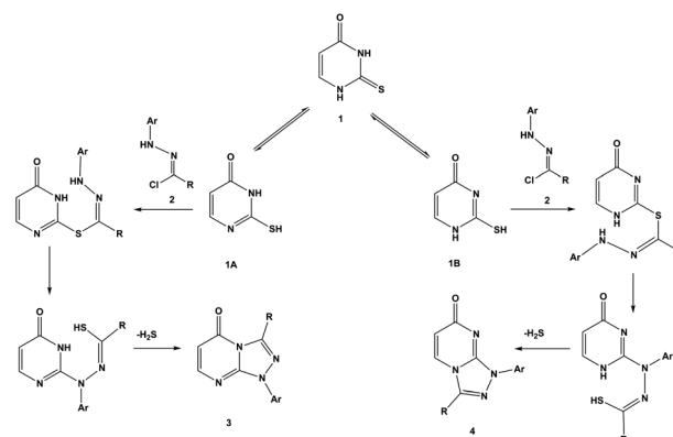
Scheme 3 Reaction pathways of thioracil 1 and hydrazonoyl chlorides 2 to form regioisomers 3 and 4 .
