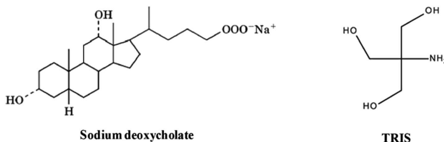
Scheme 1 Molecular structure of NaDC and Tris.
