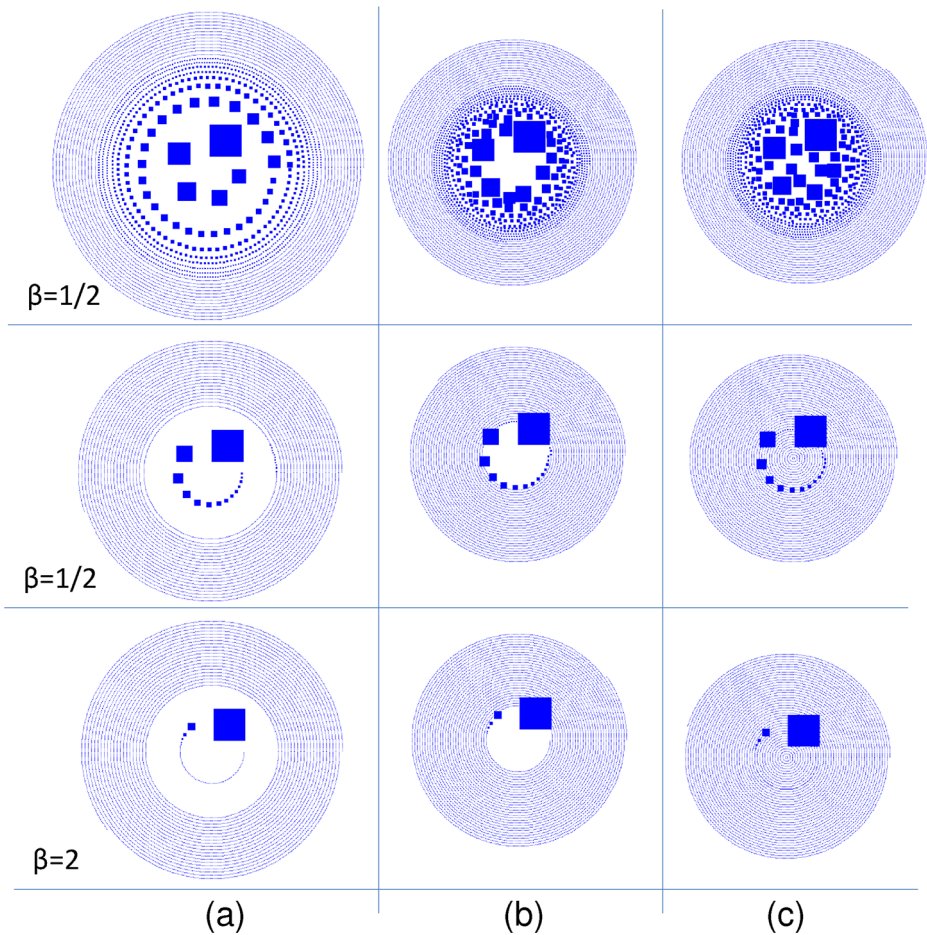
Fig. 11 (a): Concentric Spiral, (b): Concentric Spiral Ring (c): Concentric Spiral Theater over 10,000 values
