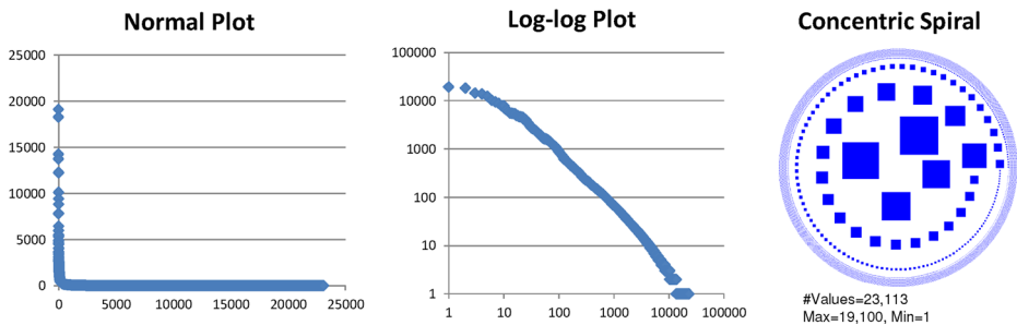
Fig. 14 The frequency of 23,113 words in Shakespeare: (a) normal, (b) log-log plot, (c) Concentric Spiral
