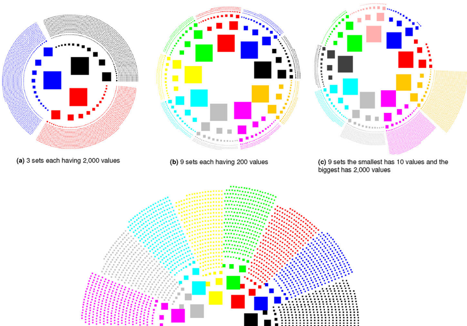
Fig. 9 Pie-chart like extension of Concentric Spiral
