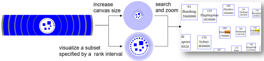
Fig. 13 10^7 values with filled rings for the very small values, and interactive options
