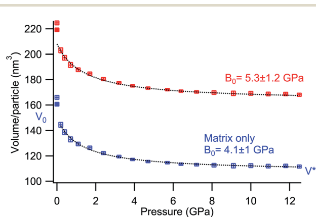
Fig. 4 (red) Volume per particle upon pressure, (blue) volume of the matrix only and (black dotted line) the fit using the Rault model.
