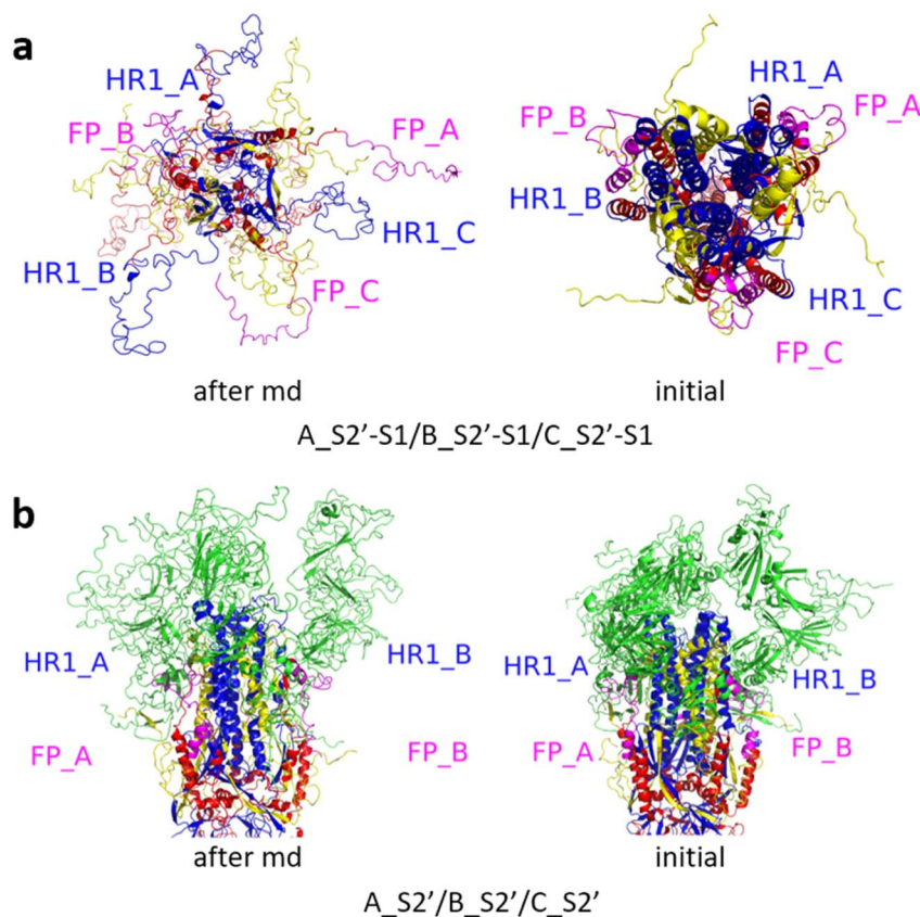
Fig. 9 (a) A_{S2'-S1}/B_{S2'-S1}/C_{S2'-S1} showed obvious outward motions of FP and HR1, and (b) A_{S2'}/B_{S2'}/C_{S2'} did not show obvious conformational changes for FP and HR1. Green represents the S1 subunit, blue for HR1, magenta for FP, yellow for residues 685–815 connecting S2 and S2' cleavage sites, and red for other residues. The MD simulations were performed using the SMOG model. 9
