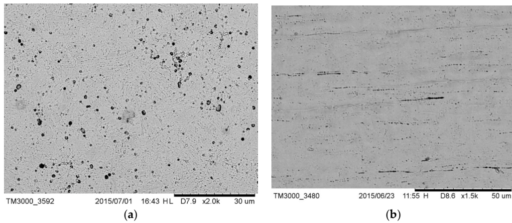
Figure 1. (a) Microstructure of drill C containing sulfide precipitates; (b) external surface of drill C; milling lines were visible.
