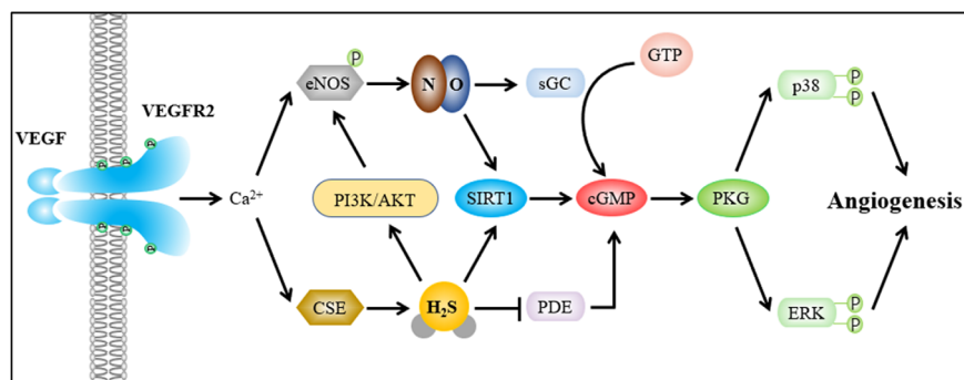
FIGURE 3 H 2 S and NO interact and depend on each other to jointly regulate angiogenesis. AKT, protein kinase B; cGMP, cyclic guanosine monophosphate; CSE, cystathionine \gamma -lyase; eNOS, endothelial nitric oxide synthase; ERK, extracellular signal-related kinases; GTP, guanosine triphosphate; sGC, soluble guanylate cyclase; SIRT1, sirtuin 1; PDE, phosphodiesterase; PI3K, phosphoinositide 3-kinase; PKG, protein kinase G; VEGF, vascular endothelial growth factor.
