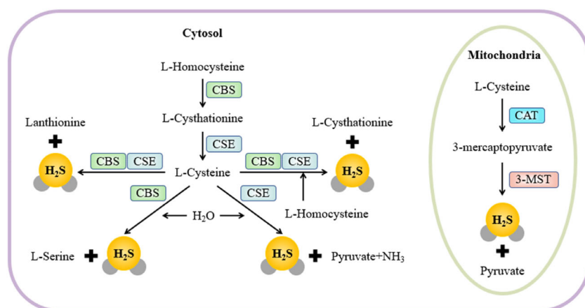
FIGURE 1 The synthesis of intracellular H 2 S. CBS, CSE, 3-MST/CAT are enzymes that catalyse the production of H 2 S in cells. CAT, cysteine aminotransferase; 3-MST, 3-mercaptopyruvate sulphurtransferase; CSE, cystathionine \gamma -lyase; CBS, cystathionine \beta -synthase.
