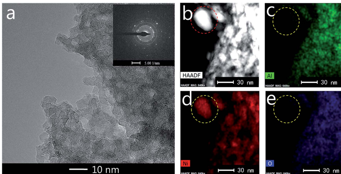
Fig. 5 (a) TEM, (b) STEM-HAADF, (c) Al map, (d) Ni map, (e) O map images of the spent 25Ni/MA catalyst.
