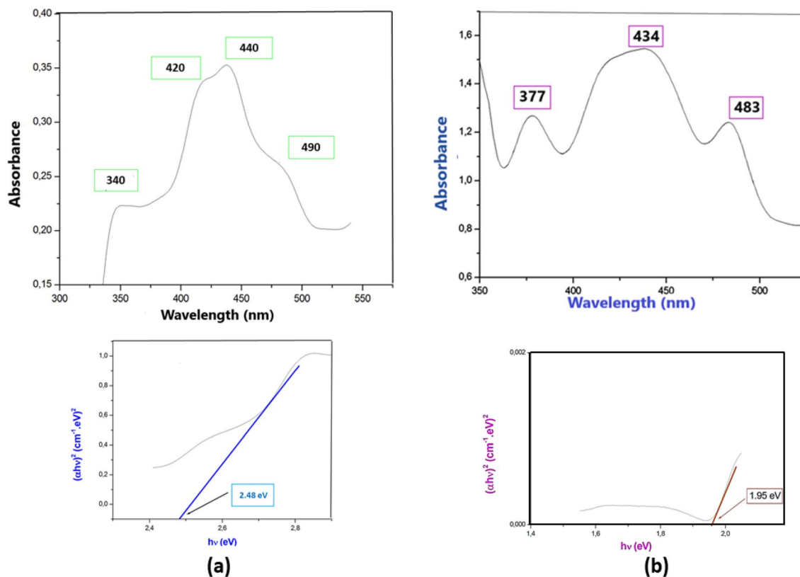
Figure 8. Solid state UV-Vis spectrum and TAUC representation of (a) [\text{Co}(\text{SCN})_4] \cdot (\text{C}_8\text{H}_{12}\text{N})_3 \cdot \text{Cl} and (b) [\text{Co}(\text{SCN})_4] \cdot (\text{C}_5\text{H}_{11}\text{N}_3)_3 \cdot 2\text{Cl} .
