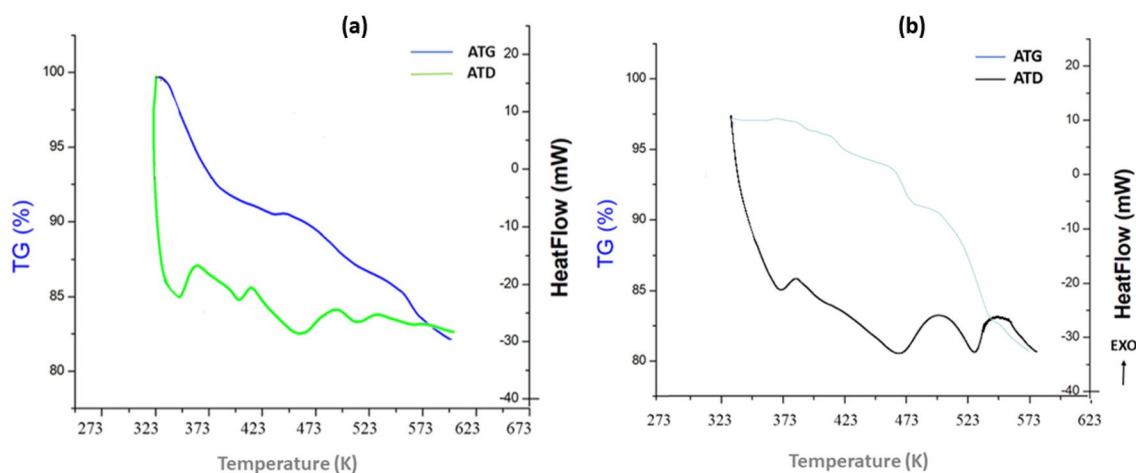
Figure 9. DTA/TG curves of (a) [\text{Co}(\text{SCN})_4] \cdot (\text{C}_8\text{H}_{12}\text{N})_3 \cdot \text{Cl} and (b) [\text{Co}(\text{SCN})_4] \cdot (\text{C}_5\text{H}_{11}\text{N}_3)_3 \cdot 2\text{Cl} .
