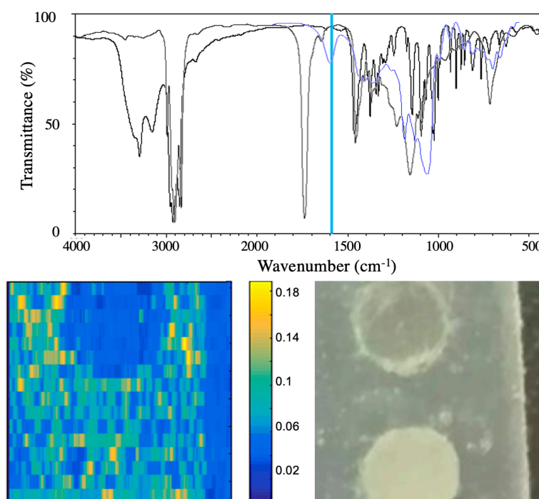
Figure 10. Top: transmittance infrared spectra of agarose (black), Intralipid ® (grey) and potato starch (blue). Bottom: images of potato starch (upper) and Intralipid ® (lower) pills in agarose matrix. Left panel shows the OF image taken at 6.2\ \mu\text{m} by raster scanning the MIR-QCL beam. Right panel shows a photo of the sample (adapted from [41]).
