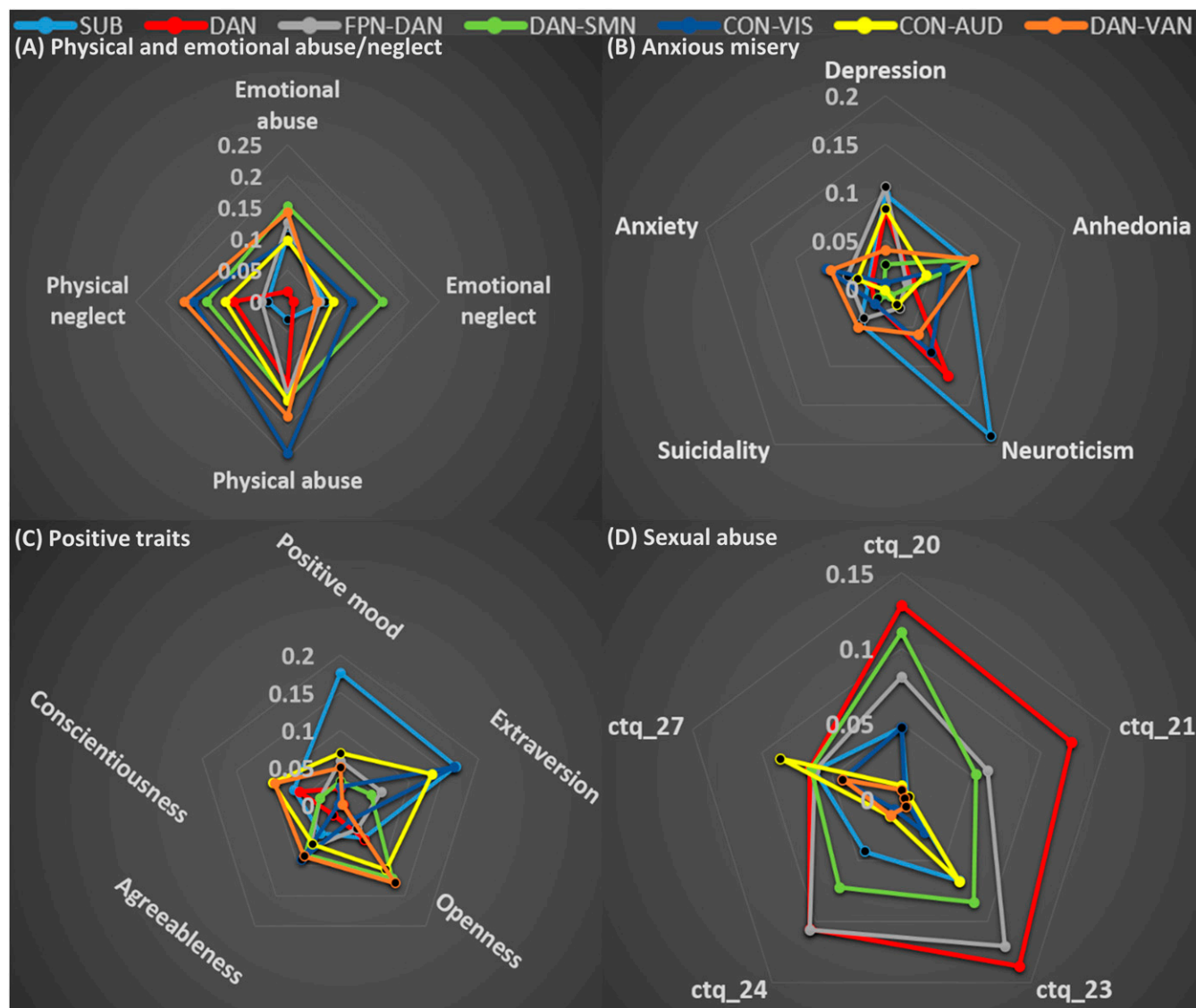
Fig. 4. Radar plots showing patterns of association of network connectivity to subsets of physical and emotional abuse and neglect ( A ), anxious misery ( B ), positive traits ( C ), and sexual abuse ( D ). The values displayed by the dots in the radar plots are the absolute values of Pearson's correlation coefficients, negative coefficients are depicted by black nodes, and a table of the values is provided in SI Appendix, Table S5 . ctq, child trauma questionnaire.
