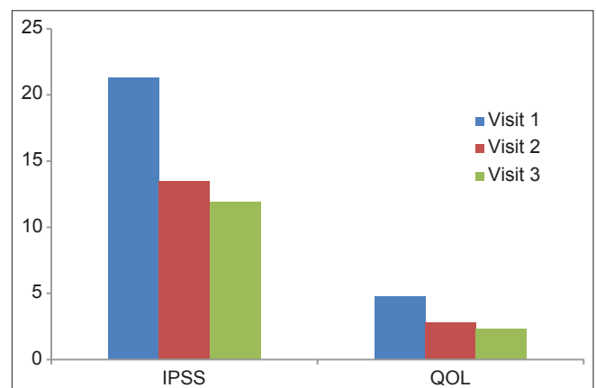
Figure 2: Variation in the IPSS QOL scores in the naftopidil group
