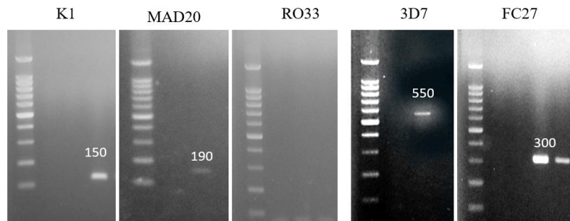
Fig. 2: Allelic variations of Pfmsp-1 and Pfmsp-2 genes based on the DNA extracted from RDT cartridges and GSBS, are showing a 150 bp in K1, 190 bp in MAD20, and negative in RO33 of Pfmsp-1 allelic family, a 550 bp of 3D7 and 300 bp of FC27 of Pfmsp-2 allelic family
