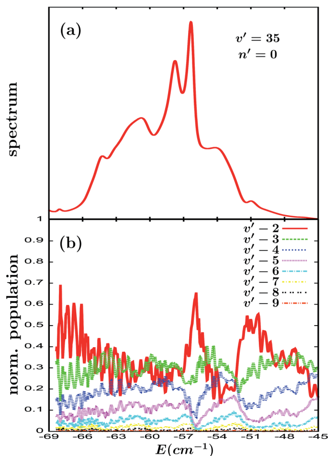
Fig. 5 (a) Excitation spectrum of the Ne-Br 2 (B, \nu' = 35 ) ground intermolecular resonance. (b) Asymptotic normalized Br 2 (B, \nu_f ) fragment vibrational populations in the \nu_f = \nu' - 1, \dots, \nu' - 9 final vibrational state, upon the predissociation of the Ne-Br 2 (B, \nu' = 35 ) ground resonance state.
