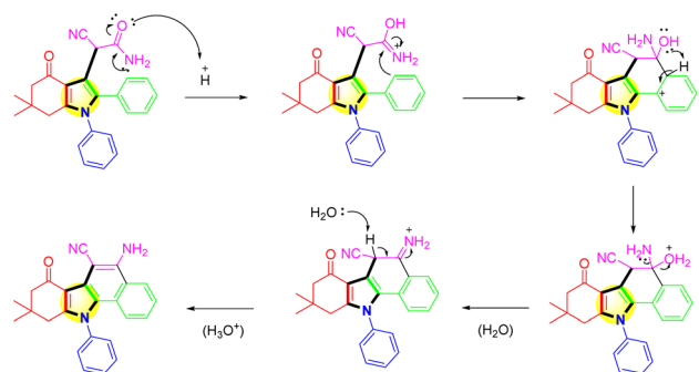
Scheme 4 Mechanism of the intramolecular cyclization of 3-cyanoacetamide pyrrole over the AC-SO 3 H catalyst.
