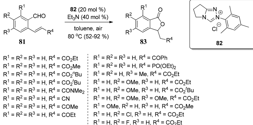
Scheme 11 NHC-catalyzed domino oxidation/oxa-Michael addition of 2-alkenylbenzaldehydes.
