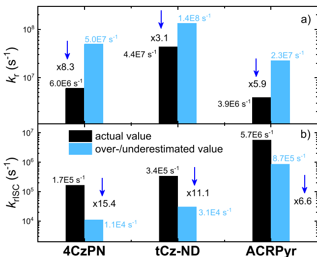
Figure 4. (a) Fluorescence radiative decay and (b) reverse intersystem crossing rates for compounds 4CzPN, tCN-ND, and ACRPyr. Accurate values are shown as black bars, and inaccurate values are shown as blue bars. The numbers close to the arrows denote the ratio between both values. k_{rISC} was calculated according to the models used in the initial reports. k_{rISC} of 4CzPN was calculated according to Kreiza et al. 8
