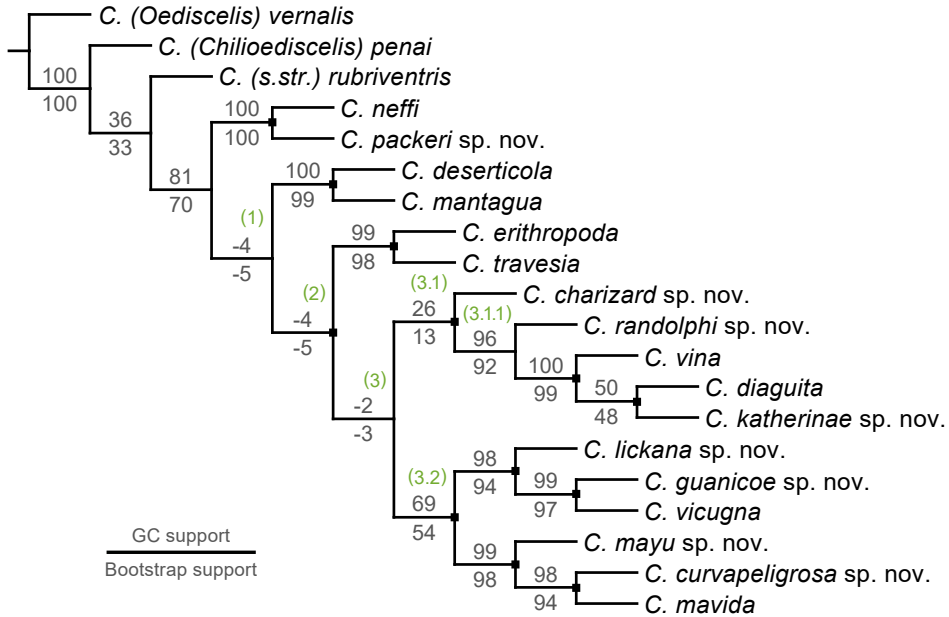
Figure 51. Single most parsimonious tree resulting from maximum parsimony analysis of combined morphological and molecular dataset. GC support values are indicated above branches, bootstrap support values are below. Nodes with distributional disjunctions are indicated by a black square. Numbered groups are discussed in text.
