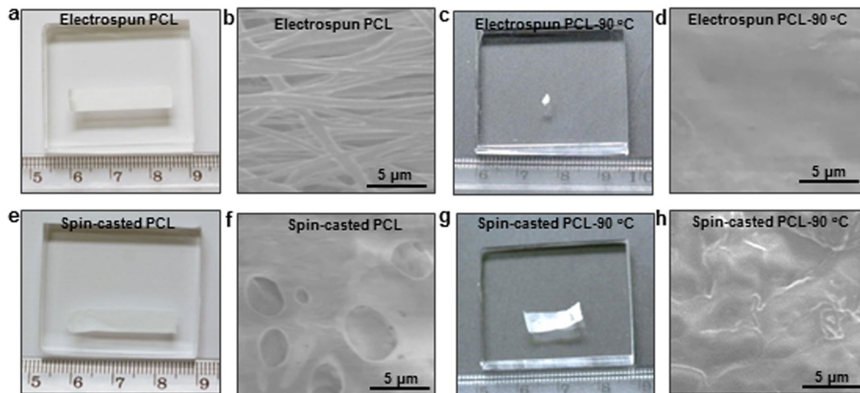
Figure 1. Heat induced shrinkage of electrospun PCL nanofibrous polymer film. (a) An optical and (b) SEM images of an electrospun PCL nanofibrous polymer film. (c) Electrospun PCL nanofibrous polymer film after heated at 90 °C. (d) SEM images of the electrospun PCL nanofibrous polymer film after heating. (e) Optical and (f) SEM images of spin-casted PCL film. (g) Spin-casted PCL film after heated at 90 °C. (h) SEM images of the spin-casted PCL film after heating.
