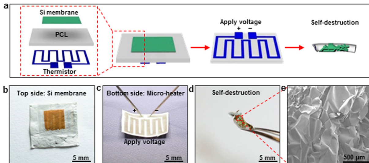
Figure 5. On-demand destruction of Si membrane on electrospun PCL nanofibrous polymer film. (a) Schematic illustration of the on-demand self-destruction of Si membrane on an electrospun PCL nanofibrous polymer film. (b,c) Optical images of both sides of a self-destructive device consisting of an integrated resistor with the electrospun PCL nanofibrous polymer film and Si membrane. (d) Optical image of a self-destructed device after applying electrical power on the resistor. (e) An SEM image of the fragmented Si membrane.
