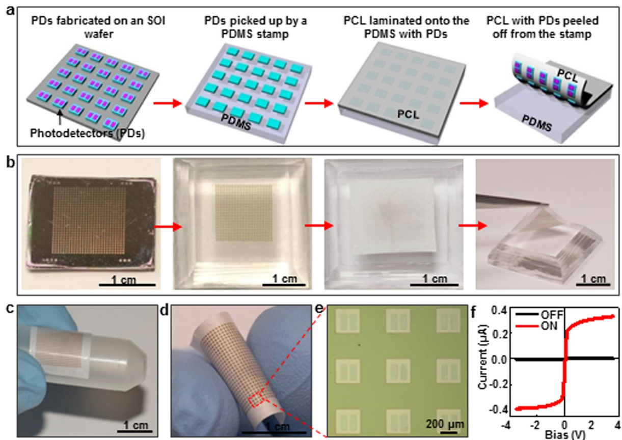
Figure 2. Fabrication and characterization of Si-based photodetectors on electrospun PCL nanofibrous polymer film. (a) Schematics and (b) photographs illustrating the fabrication process of Si-based photodetectors on an electrospun PCL nanofibrous polymer film. (c,d) Photographs demonstrating the flexibility of the device. (e) Optical image of the photodetector arrays. (f) Device performance of the photodetectors on the electrospun PCL nanofibrous polymer film.
