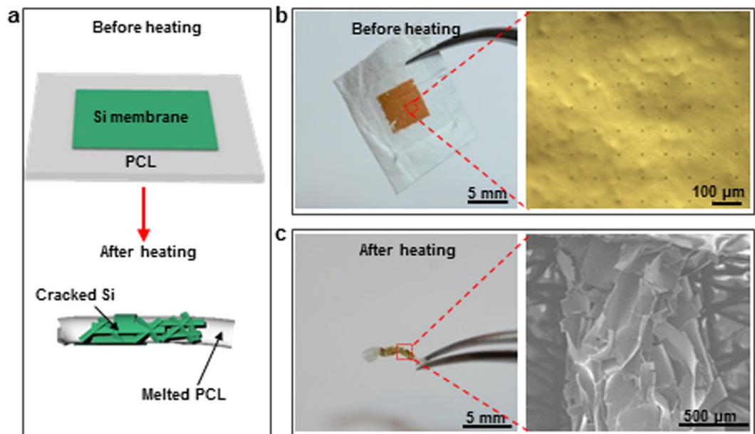
Figure 4. Thermal triggered destruction of Si membrane on electrospun PCL nanofibrous polymer film. (a) Schematic illustration of the destruction behavior of Si membrane on an electrospun PCL nanofibrous polymer film triggered by heating. Images of the Si membrane on an electrospun PCL nanofibrous polymer film (b) before and (c) after heating.
