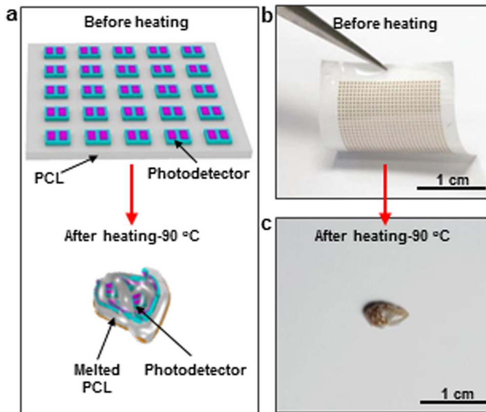
Figure 3. Thermal triggered destruction of Si-based photodetectors on electrospun PCL nanofibrous polymer film. (a) Schematic illustration of the destruction behavior of Si-based photodetectors on an electrospun PCL nanofibrous polymer film triggered by heating. Photographs of the Si-based photodetectors on an electrospun PCL nanofibrous polymer film (b) before and (c) after heating.
