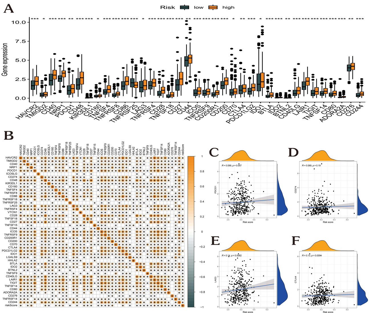
Figure 6 Correlational analysis of risk score with 46 GC common immune checkpoint genes. (A) Differential expression of the 46 immune checkpoint genes between high- and low-risk score groups. (B) Correlation of risk score with 46 immune checkpoint genes in GC. (C–F) Correlation of risk score with the expression of PDCD1, CD274, LAG3, and CTLA4 in TCGA-GC dataset. (* p < 0.05 ; ** p < 0.01 ; *** p < 0.001 ).
