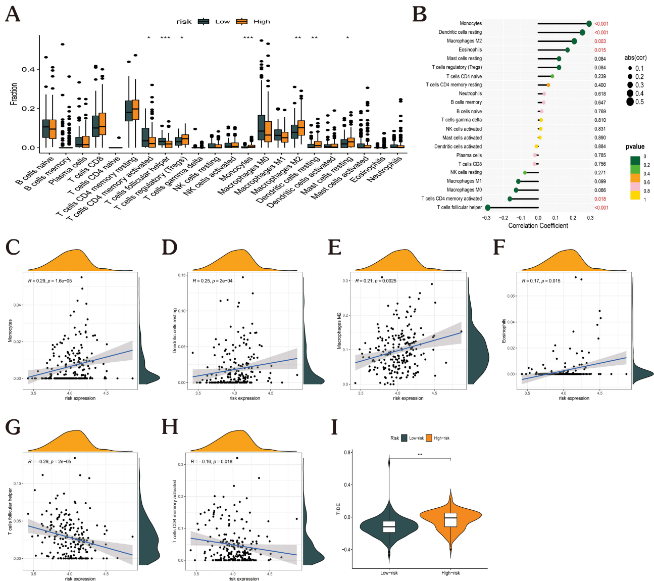
Figure 7 Link between risk score and immune cell infiltration. (A) Box plots showing the differences in the proportions of 22 different types of immune cells in GC tumor samples between high- and low-risk groups. (B) Correlation between risk score and 22 immune cell types in GC ( p < 0.05 in red). (C–H) Correlation of risk score with (C) monocytes, (D) dendritic cells resting, (E) macrophages M2, (F) eosinophils, (G) T cells CD4 memory activated, and (H) T cells follicular helper in GC. (I) Assessment of immune evasion efficacy in the high- and low-risk-expression groups. (* p < 0.05 ; ** p < 0.01 ; *** p < 0.001 ).
