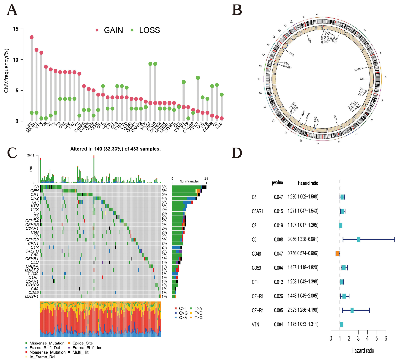
Figure 2 Molecular characterization and expression variants of complement family genes in GC. (A) Analyzing the frequencies of CNV in the complement family of genes in GC. The frequencies of deletions are shown by green dots, red dots represent amplification frequencies, and alteration in frequency is depicted by the column height. (B) Location of complement family gene CNV on 23 chromosomes. (C) The frequency of mutations in genes belonging to the complement family in 433 TCGA patients with GC. TMB is represented by the top bar, and each column denotes a single patient. In addition, each regulator’s mutation rate is shown to the right in the figure. The visual representation of the distribution of different types of regulatory systems is shown on the bar graph to the right. The percentage of conversions in each group is shown as a stack of horizontal bars. (D) The genes of the complement family were examined utilizing a univariate Cox regression analysis.
