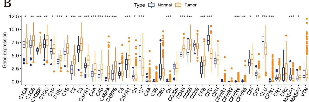
Figure 1 Expression of complement family genes and three classical pathways of the complement system. (A) Three classical pathways of the complement system. (B) Expression of 42 complement genes in normal gastric tissue (dark blue) and tumor tissue (dark Orange). Interquartile ranges are shown by box plots. Boxed rows represent medians, and P-values are depicted by asterisks (* p < 0.05; ** p < 0.01; *** p < 0.001).
