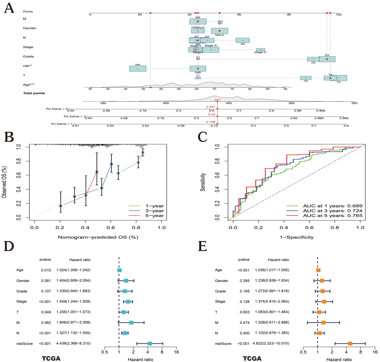
Figure 4 Developing a nomogram and analyzing prognostic factors. (A) A nomogram model was constructed to predict the 1-, 3-, and 5-year OS probabilities of patients with GC. (B) Nomogram model-related calibration curves for estimating 1-, 3-, and 5-year OS for GC patients. (C) Nomogram model-related ROC curves for estimating 1-, 3-, and 5-year OS for GC patients. (D–E) The results of univariate (D) and multivariate Cox regression (E) for the OS of patients with EC are shown in forest plots. (**p < 0.01; ***p < 0.001).
