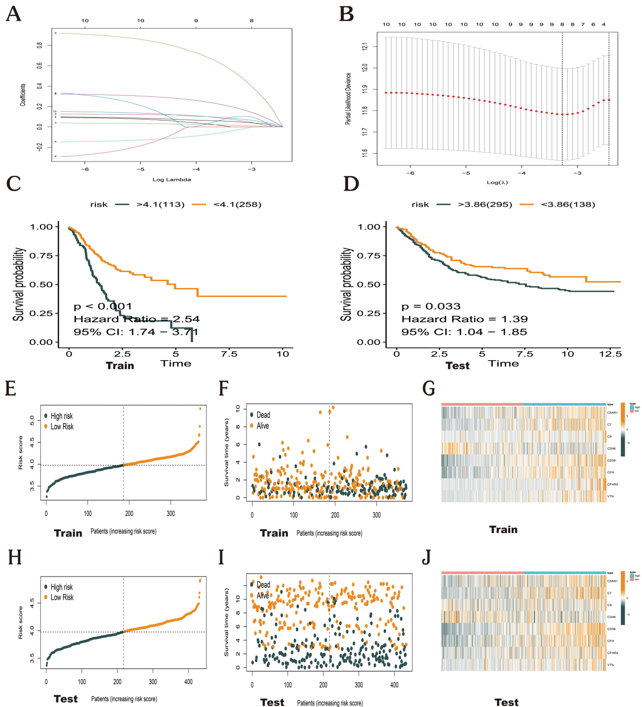
Figure 3 Construction of a prognostic model based on complement family genes. (A) The log (lambda) sequence is shown against the Lasso coefficient profiles of the 10 genes chosen for the OS analysis. (B) The 10-fold cross-validation error (the minimal error is represented by the first vertical line, and the error within 1 standard error of the minimal is represented by the second vertical line). (C and D) Survival probabilities for patients with high-risk score in contrast with those with low-risk score, as shown by Kaplan-Meier plots. (E–G) Distribution of risk scores, associated survival data, and expression of eight core genes in the TCGA cohort. (H–J) Distribution of risk scores, associated survival data, and expression of eight core genes in the GSE84437 cohort.
