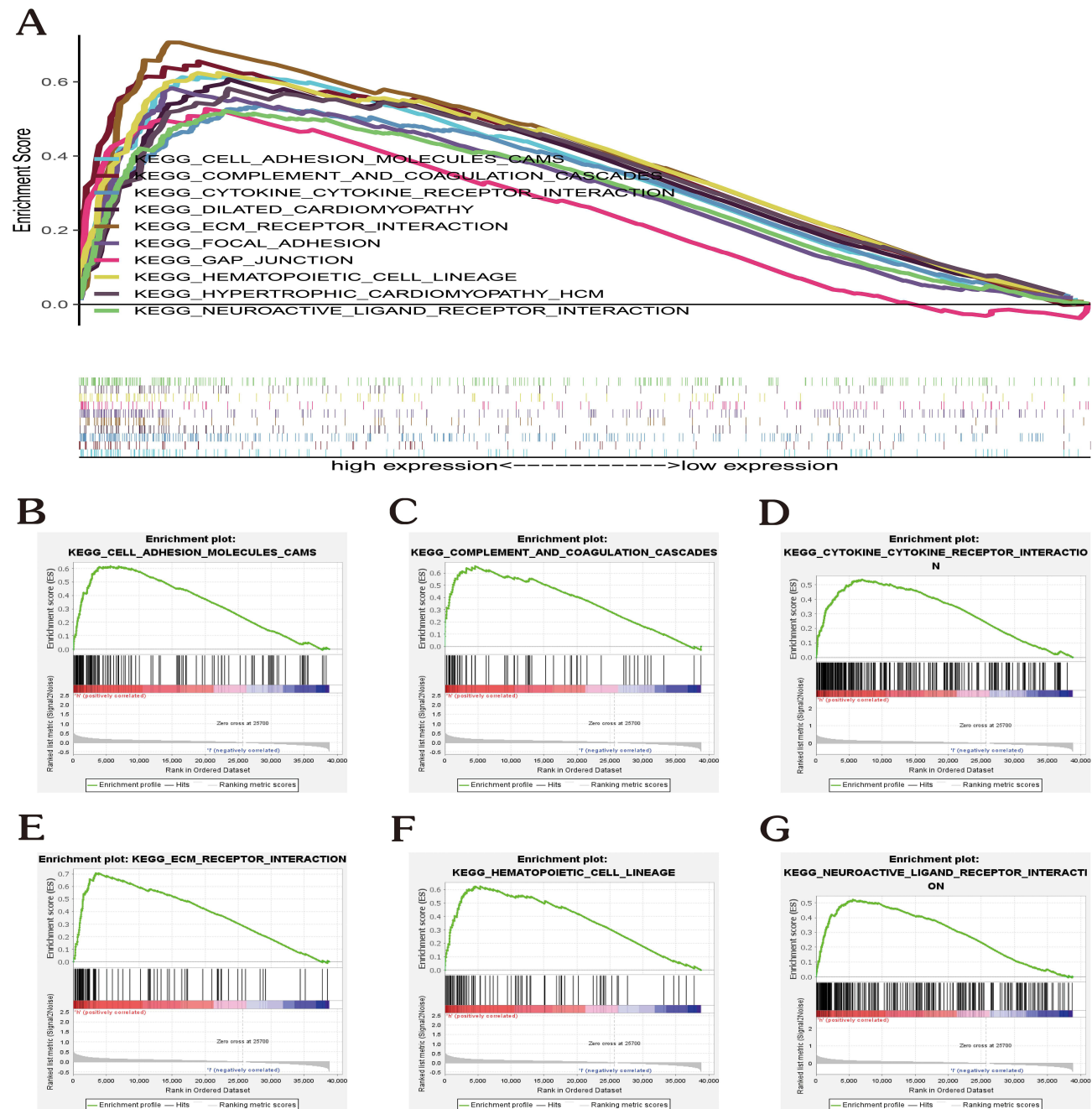
Figure 5 Gene set enrichment analysis. (A) Top 10 pathways related to risk score-associated gene enrichment. (B) Cell adhesion molecules cams. (C) Complement and coagulation cascades. (D) Cytokine cytokine receptor interaction. (E) Ecm receptor interaction. (F) Hemopoietic cell lineage. (G) Neuroactive ligand receptor interaction.
