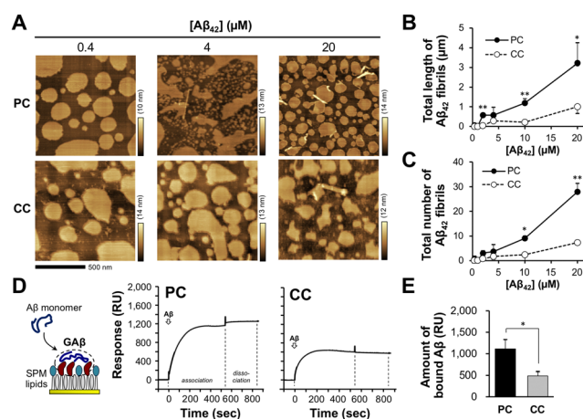
Fig. 2 Binding and accumulation of A \beta_{42} on reconstituted SPM lipid membranes. (A) Typical AFM images of the reconstituted lipid bilayer with SPM lipids extracted from the precuneus (PC) and cortex of calcarine (CC) after incubation with A \beta_{42} (0.4–20 \mu\text{M} ) at 37 °C for 15 min. (B) and (C) Total length (B) and number (C) of observed A \beta_{42} fibrils on the membrane after A \beta_{42} interaction for 15 min. * p < 0.05 , ** p < 0.01 compared with CC. (D) Typical SPR sensorgrams of A \beta_{42} (20 \mu\text{M} ) against the reconstituted lipid monolayer. Sensorgrams for an association time of 540 s and dissociation time of 300 s are shown. (E) Amount of A \beta_{42} bound to the lipid monolayer. The response value (RU) at 840 s was used as the amount of bound A \beta_{42} . * p < 0.05 . Data are presented as average values \pm standard deviation ( n = 3 ).
