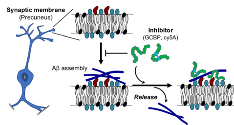
Fig. 8 Proposed model of the release of A \beta 42 assemblies on the synaptic membrane by ganglioside nanocluster-targeting inhibitors.
