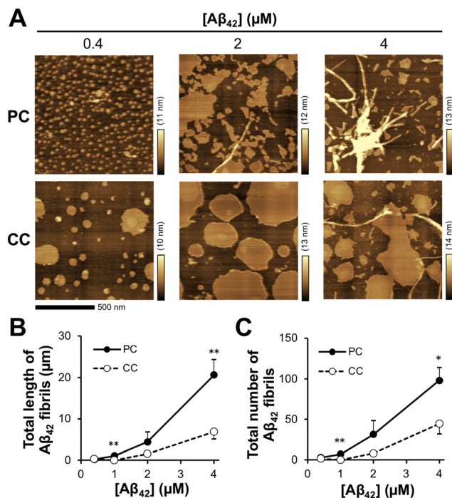
Fig. 3 A \beta_{42} fibril generation on the SPM lipid membrane. (A) Typical AFM images of the reconstituted lipid bilayer with SPM lipids extracted from PC and CC after incubation with A \beta_{42} (0.4–4 \mu\text{M} ) at 37 °C for 24 h. (B) and (C) Total length (B) and number (C) of observed A \beta_{42} fibrils on the lipid bilayer after A \beta_{42} interaction for 24 h. * p < 0.05 , ** p < 0.01 compared with CC. Data are presented as average values \pm standard deviation ( n = 3 ).
