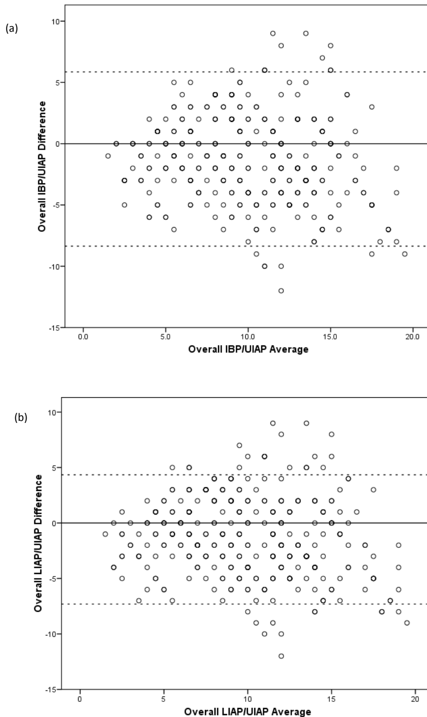
Figure 4 Intra-bladder pressure (IBP) and upper intra-abdominal pressure (UIAP), and lower intra-abdominal pressure (LIAP) and UIAP. (a) Bland and Altman plot to compare IBP and UIAP with a supine body position and a head of bed position of 30°. (b) Bland and Altman plot to compare LIAP and UIAP with a supine body position and a head of bed position of 30°. LLA and ULA marked by dotted lines.
