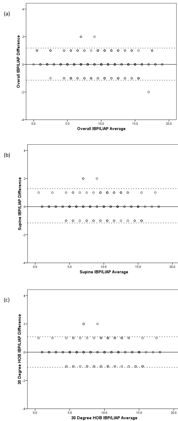
Figure 3 Bland and Altman plots comparing intra-bladder pressure (IBP) and lower intra-abdominal pressure (LIAP). (a) Bland and Altman plot to compare IBP and LIAP with a supine body position and a head of bed position of 30°. (b) Bland and Altman plot to compare IBP and LIAP with a supine body position. (c) Bland and Altman plot to compare IBP and LIAP with a head of bed position of 30°. Lower level of agreement (LLA) and upper level of agreement (ULA) marked by dotted lines.
