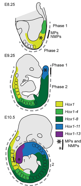
Figure 3. Early temporal collinearity of Hox gene transcription is relayed by the axial progenitors into spatially collinear expression domains in the emerging differentiated tissues. (E8.25) The transcript domains of Hox1 followed by that of Hox2 to Hox4 (phase 1, temporal collinearity) expand anteriorly and reach the axial progenitor region ([*] MPs and NMPs) before expanding further anteriorly during phase 2. (E9.25) Transcriptional initiation of the next Hox genes has occurred (mid-trunk Hox4 to Hox8 ), and activation of more posterior Hox genes takes place (as shown with Hox11 ). The expression domains expand anteriorly toward the axial progenitor area in those tissues generated by the descendants of the MPs and NMPs (phase 2, spatial collinearity). (E10.5) Hox13 is now transcriptionally activated and expressed strongly posteriorly, where it counteracts further axial extension. The Wnt and Fgf pathways are weakened, and the progenitor niche becomes deficient, with fewer and fewer MPs and NMPs (smaller asterisk). The color code identifies the combinations of Hox genes expressed along the axis at the different stages. MPs and NMPs are found around the anterior part of the primitive streak, just posterior to the node (indentation) at E8.25 and in the tailbud at E9.25 and E10.5. For the E8.25 embryo, anterior is to the left; for the E9.25 and E10.5 embryos, anterior is to the top.
