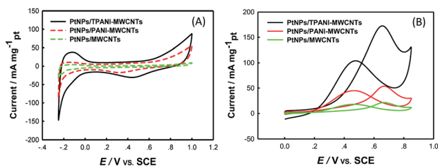
Fig. 5 CVs of PtNPs/MWCNTs/GCE, PtNPs/PANI-MWCNTs/GCE, PtNPs/TPANI-MWCNTs/GCE in N_2 -saturated 0.5 M H_2SO_4 (A) and in N_2 -saturated 0.5 M H_2SO_4 + 1.0 M CH_3OH (B) at a scan rate of 50 \text{ mV s}^{-1} .
