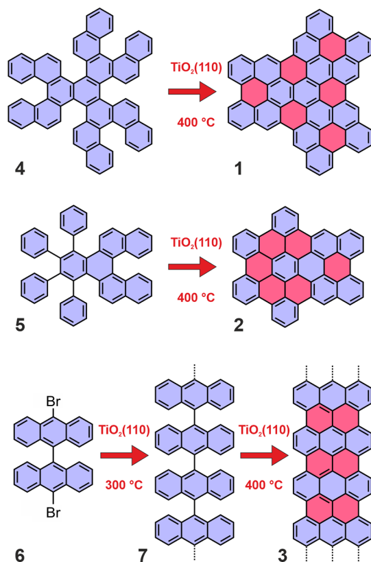
Figure 1. Schematic illustration of synthetic paths providing nanographenes 1 and 2, 7-AGNR (3), and DBBA-based polymers (7) on \text{TiO}_2(110)-(1\times 1) from the corresponding molecular precursors (i.e., 4, 5, and 6). The red color represents additional six-membered rings fabricated in the on-surface experiments.
