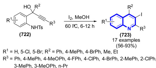
Scheme 203 Synthesis of 3-iodoquinolines catalyzed by iodine.
