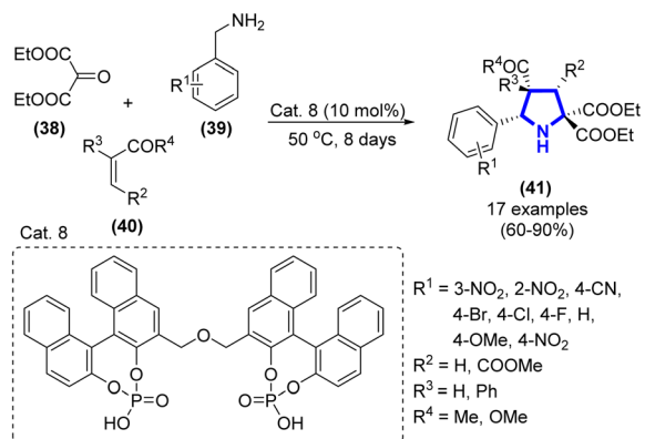
Scheme 11 Synthesis of pyrrolidine derivatives catalyzed by Cat. 8 .
