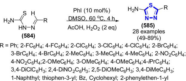
Scheme 157 Synthesis of 2-amino-1,3,4-thiadiazole catalyzed by PhI.
