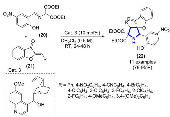
Scheme 5 Synthesis of pyrrolidine derivatives catalyzed by Cat. 3.
