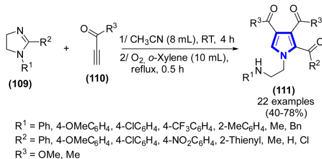
Scheme 30 Synthesis of polysubstituted pyrroles.
