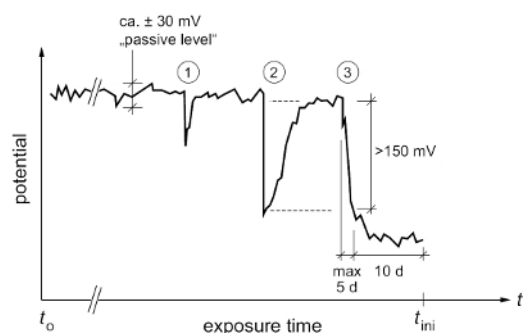
Figure 3. Schematic Drawing of Possible Time-evolutions of the Steel Potential that Illustrates the Criterion for Corrosion Initiation. At point 1, a potential drop by less than 150 mV from the initial "passive level" occurs; at point 2, a potential drop by at least 150 mV occurs, which is followed by repassivation; at point 3, a potential drop of at least 150 mV occurs (within a max. of 5 days) and the achieved negative potential level is sustained over 10 days. At t_{ini} , withdraw the sample from the exposure solution. Please click here to view a larger version of this figure.
