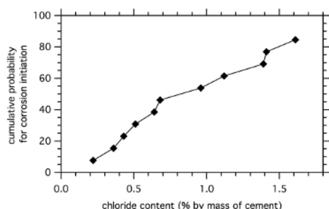
Figure 8. Example of C_{crit} Measured in 11 Samples Taken from Within a Small Concrete Area in a More than 40 Years Old Road Tunnel in the Swiss Alps. Please click here to view a larger version of this figure.
