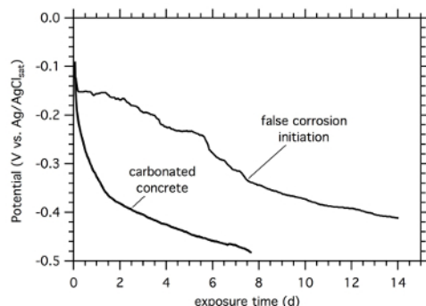
Figure 9. Examples of Marked Potential Decreases Immediately upon Exposure in Chloride-free Solution. In one case, the concrete at the steel depth was already carbonated, thus upon arrival of water at the steel surface, the corrosion process immediately started, leading to a sharp decrease in potential. In the other case, false corrosion initiation occurred at one of the steel bar ends, which here led to a more gradual potential decrease. Please click here to view a larger version of this figure.
