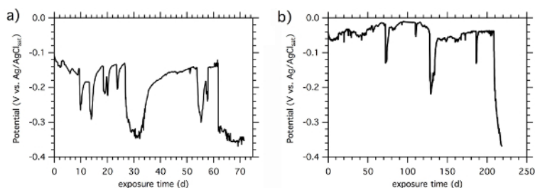
Figure 7. Representative Examples of Measured Potential vs. Time Curves. The typically pronounced potential drops that may be followed by a potential increase (repassivation) until stable corrosion initiation according to the suggested criterion finally initiates. (a) Shows a case where the potential stabilizes on the negative level, and (b) is an example where the potential continues decreasing over the studied period of 10 days. Please click here to view a larger version of this figure.
