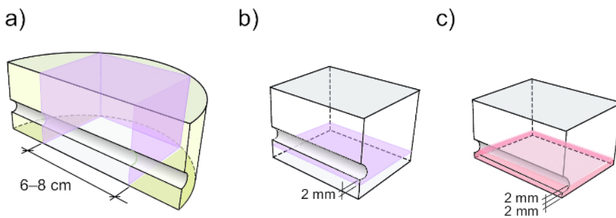
Figure 6. Schematic Drawing Illustrating the Sampling for the Chloride Analysis After Corrosion Initiation: (a) removal of epoxy-coated parts of the split concrete core (purple = cutting planes); (b) removal of the concrete cover down to 2 mm from the steel surface (purple = cutting plane); (c) grinding over a depth interval of \pm 2 mm of the steel bar cover depth (red = sampled volume). Please click here to view a larger version of this figure.
