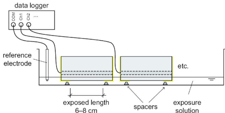
Figure 2. Schematic Drawing of the Setup for the Corrosion Test in the Laboratory. This shows the placement of the samples in the exposure tank. Spacers are used to ensure contact to exposure solution from the bottom sample surface. All samples are connected to a data logger, measuring the potential of each sample vs. a reference electrode placed in the exposure solution. Please click here to view a larger version of this figure.
