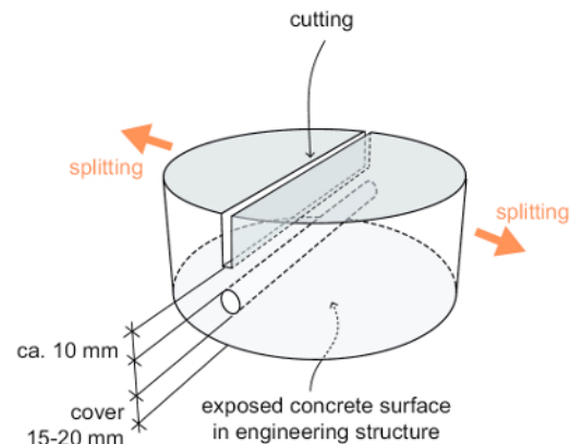
Figure 4. Schematic Drawing Illustrating the Cutting and Splitting of the Concrete Sample after Detection of Corrosion Initiation. First, a "trench" is cut from the rear side, in parallel to the steel bar. By inserting a chisel or a similar tool, the trench can be used to split the sample as indicated by the arrows. Please click here to view a larger version of this figure.
