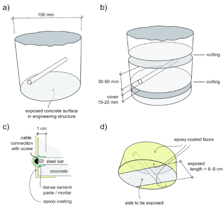
Figure 1. Schematic Drawing of the Sample Taken from a Structure and Treated in the Laboratory: (a) concrete core with an embedded piece of reinforcing steel; (b) reducing the concrete cover on the exposed side and on the back side by water-cooled diamond cutting; (c) steel bar end protection by means of removing some concrete around the steel and replacing it with a dense cement paste/mortar and subsequent epoxy coating; and (d) epoxy-coating on lateral faces and on end zones of the exposed concrete surface. Please click here to view a larger version of this figure.
