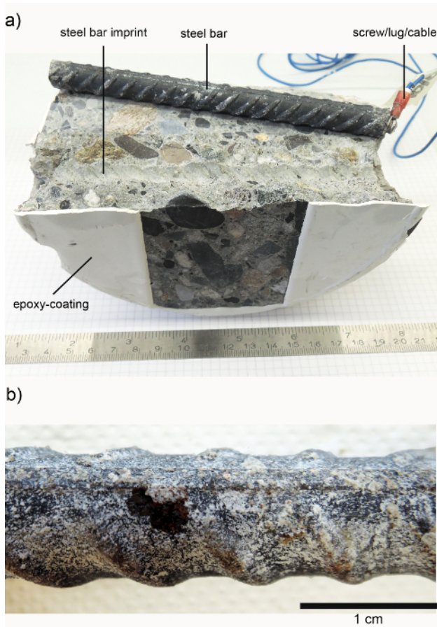
Figure 5. Photographs Illustrating Sample Analysis After Corrosion Initiation. (a) The two halves of the sample after splitting, and (b) a rust spot is visible at the steel surface after corrosion initiation. Photographs from different samples. Please click here to view a larger version of this figure.
