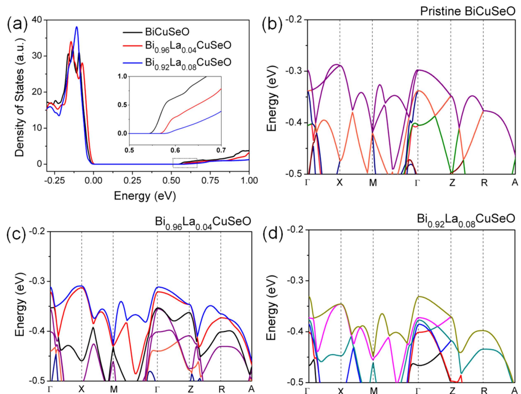
Figure 4. (a) Total density of state near the Fermi level and (b–d) the valence band maximum of \text{Bi}_{1-x}\text{La}_x\text{CuSeO} with increasing La content.
