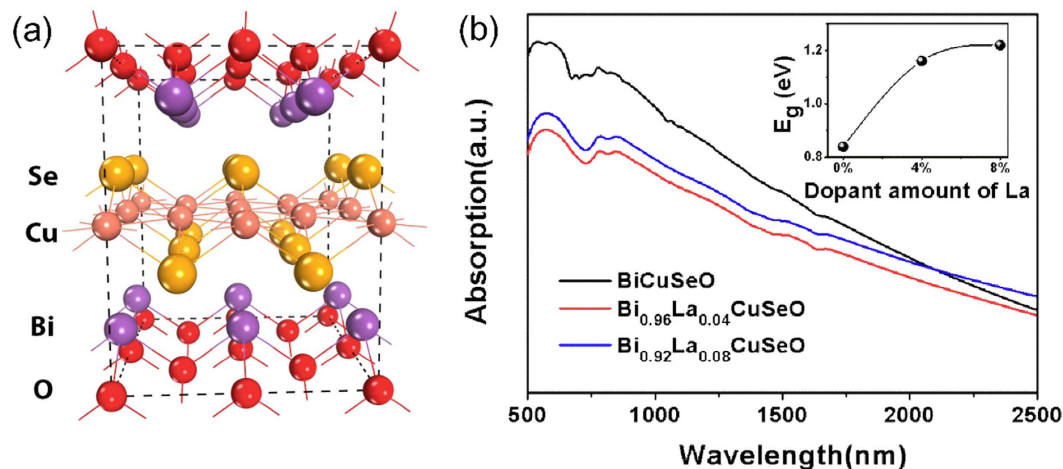
Figure 1. (a) The crystalline structure of La-doped BiCuSeO used in DFT calculations. (b) UV-Vis-NIR absorbance spectra of \text{Bi}_{1-x}\text{La}_x\text{CuSeO} ( x = 0, 0.04, 0.08 ) powder samples. Insert shows the variation of bandgaps with different La doping content estimated by Kubelka-Munk transformation.
