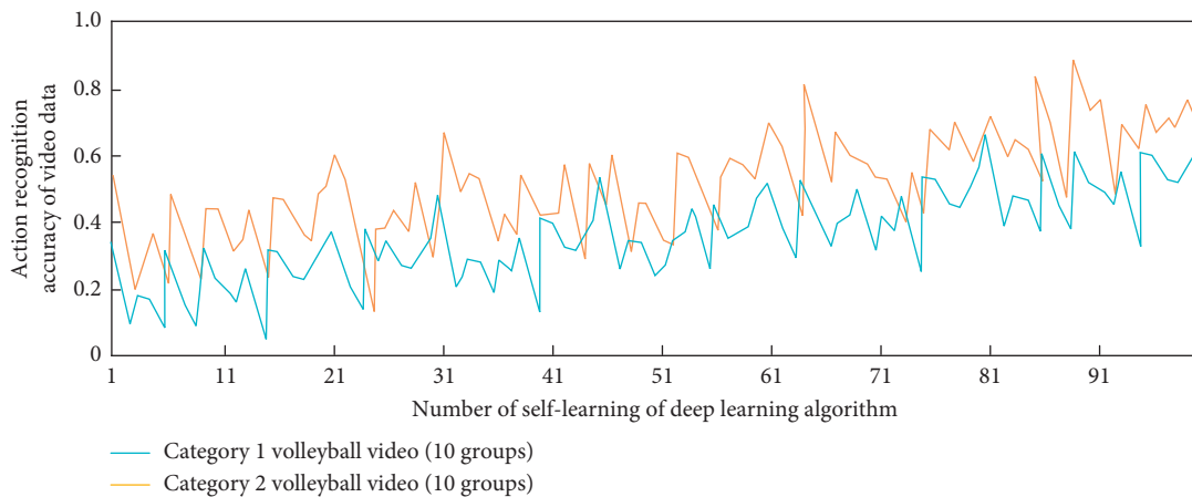
FIGURE 6: The process of simulation analysis of the accuracy of action recognition in volleyball sports videos after introducing key factors.
