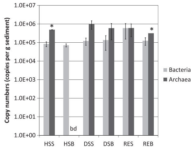
Fig. 3. Comparison of bacterial and archaeal 16S rRNA genes copy numbers. *data which were not detected in one sample of triplicate experiments. bd, below detection limit of 1.7 \times 10^3 copies. Error bars showing standard deviation.
