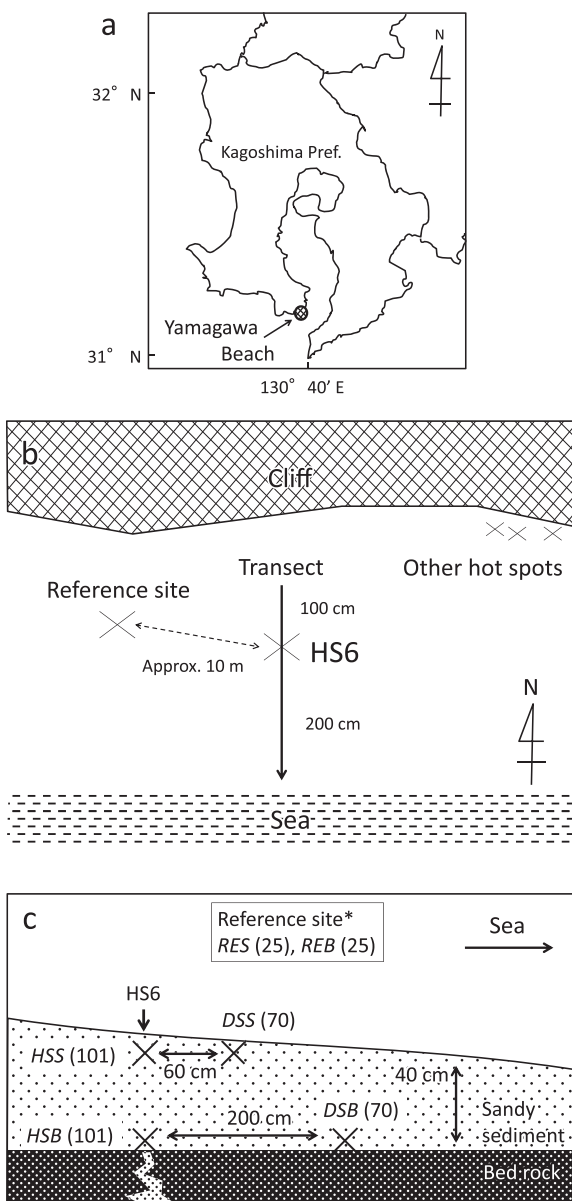
Fig. 1. Location of Yamagawa Beach (a), transect across HS6 (b), and sampling sites in the Yamagawa coastal hydrothermal field (c). Sampling sites are shown in italic. See text for abbreviations. Numbers in parentheses indicate the temperature of the samples. *Reference site is off the transect, approximately 10 m from HS6.
