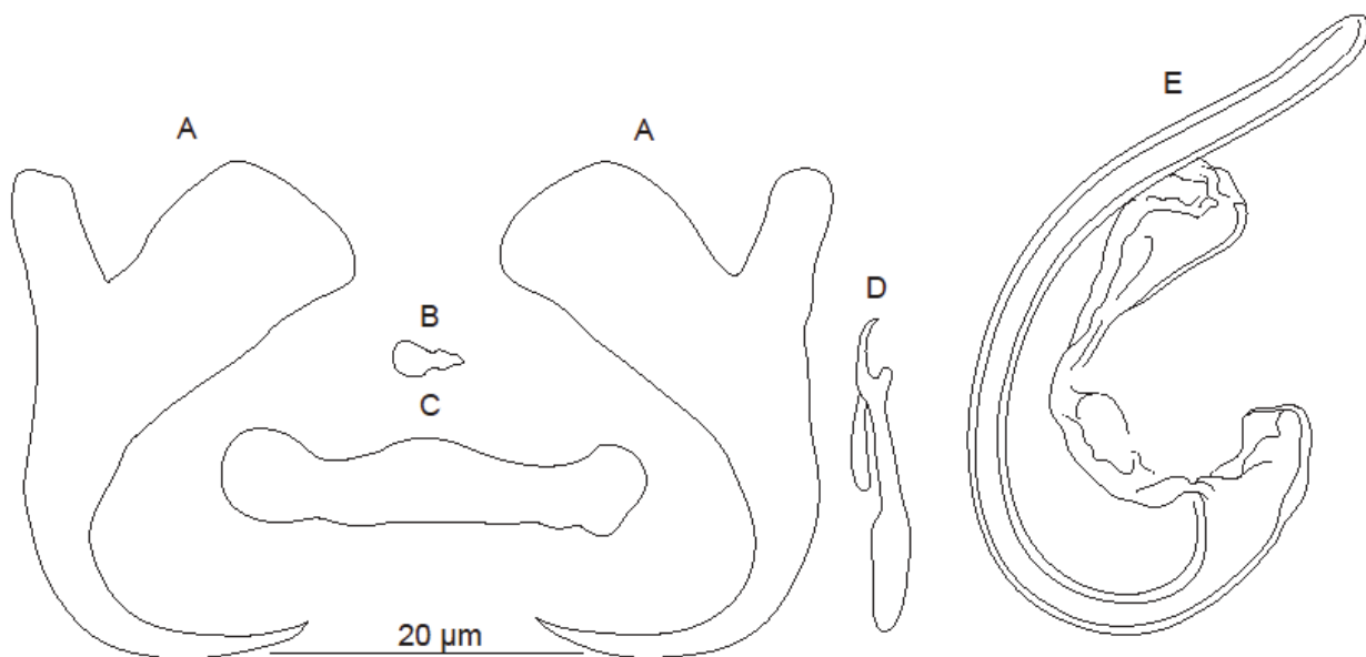
Fig. 1. Dactylogyryrus nathaliae Guégan, Lambert & Euzet, 1988. A = anchor; B = ventral bar; C = dorsal bar; D = hook; E = copulatory organ
