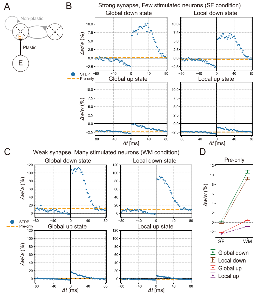
Fig. 4. STDP in different sleep states. (A) The schematic description of the simulation. Presynaptic neurons had a feedforward projection onto an excitatory postsynaptic neuron in the E1 population. The feedforward synaptic weights were plastic, whereas the recurrent synaptic weights were fixed. (B) The synaptic changes caused by the STDP stimulations (blue points) and pre-only stimulations (orange dotted lines) during each sleep state in the case of strong synapses ( w_j^{\text{ext}} = 0.5 mV) and few stimulated neurons ( N^{\text{ext}} = 20 ) (SF condition). As the value of \Delta t increased or decreased, the synaptic changes by the STDP stimulations converged to the change by the pre-only stimulations. The amount of synaptic changes follows global down > local down > global up > local up, in descending order. (C) The synaptic changes caused by the STDP stimulations (blue points) and pre-only stimulations (orange dotted lines) during each sleep state in the case of weak synapses ( w_j^{\text{ext}} = 0.09 mV) and many stimulated neurons ( N^{\text{ext}} = 40 ) (WM condition). The synapses tend to be potentiated even in up states, while the amount of synaptic changes follows global down > local down > global up > local up, in descending order, as with (B). Note that the scale is different from (B). (D) The synaptic changes caused by the pre-only stimulations. The synaptic changes were dominated by synaptic potentiation in the WM condition. Especially in the WM condition, the pre-only stimulations during global and local up states induced synaptic potentiation and depression, respectively.
