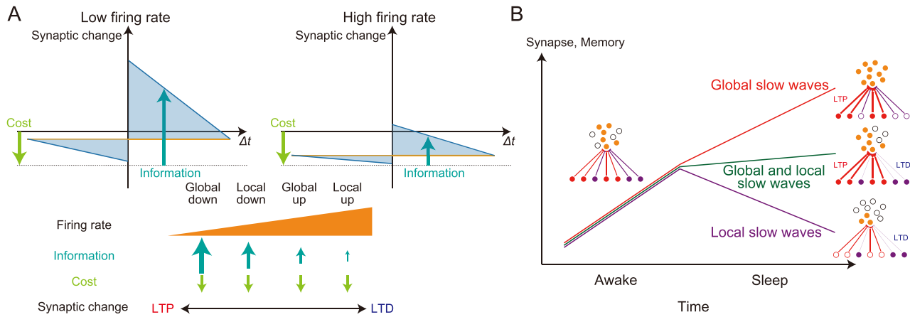
Fig. 6. The proposed role of NREM sleep is to bridge neural information coding, synaptic plasticity, and memory reorganization. (A) The relationship between the mean firing rate and synaptic changes by the infomax rule. Synaptic potentiation by the information term was decreased at a high firing rate owing to many background spikes, whereas synaptic depression by the cost term was unaffected. Therefore, the high firing rate induced synaptic depression. Because the mean firing rates are global down < local down < global up < local up in ascending order, the amount of synaptic changes follows the opposite order. (B) The possible distinct roles of global and local slow waves. Reactivated patterns during global slow waves induced synaptic potentiation, whereas those during local slow waves induced synaptic depression. This could cause selective memory consolidation and forgetting of the reactivated patterns during the global and local slow waves, respectively.
