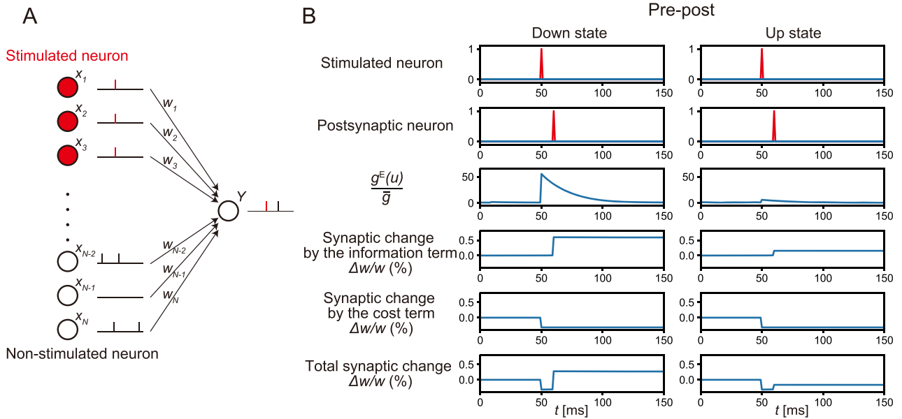
Fig. 1. The infomax rule in the single-neuron model. (A) A single-neuron model of synaptic plasticity. Stimulated neurons synchronously emit spikes upon external presynaptic stimulation, and their synaptic weights change according to the infomax rule, whereas nonstimulated neurons spontaneously emit Poisson spikes and their synaptic weights are fixed for simplicity. A postsynaptic neuron emits both spontaneous spikes and evoked spikes upon external postsynaptic stimulation. The red vertical bars represent evoked spikes. (B) Representative traces of a stimulated neuron's activity, the postsynaptic neuron's activity, the ratio of the momentary and mean activation intensity g^E(u)/\bar{g} , and changes of a synaptic weight from a stimulated neuron in the down and up states. Synaptic changes by the infomax rule were computed by summing the effects of the information term \frac{dI}{dw_j} and cost term \frac{d\Phi}{dw_j} . The synaptic increase by the information term was smaller in the up state than in the down state.
