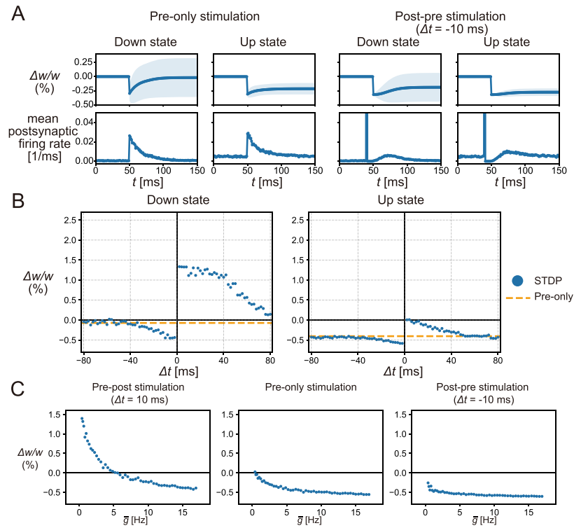
Fig. 2. The synaptic plasticity induced by the STDP stimulations. (A) The mean traces of a synaptic weight and the mean postsynaptic firing rate in the pre-only stimulations or the post-pre stimulations with \Delta t = -10 ms, where the stimulated neurons emitted a synchronous spike upon the external stimulation at t = 50 ms. In the post-pre stimulations, the postsynaptic neuron emitted an evoked spike at t = 40 ms and also responded to the presynaptic stimulation at t = 50 ms with some delay due to refractoriness. After the pre-only stimulations, the synaptic weight changed little in the down state, but was depressed in the up state. In the post-pre stimulation, the synaptic weight was depressed in both the down and up states. The lines and shadows of the weight traces represent the means and SDs, respectively. (B) The synaptic changes by the STDP stimulations (blue points) and pre-only stimulations (orange dotted lines). As the value of \Delta t increased or decreased, the synaptic changes by the STDP stimulations converged to the change by the pre-only stimulations. Synaptic plasticity was biased towards depression in the up state. (C) Synaptic changes were dependent on mean activation intensity. The synaptic changes in pre-post stimulation with \Delta t = 10 ms and pre-only stimulation decreased with increasing mean activation intensity, whereas the synaptic changes in post-pre stimulation with \Delta t = -10 ms were less sensitive to mean activation intensity.
