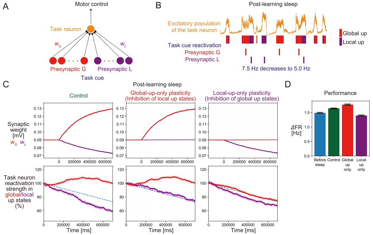
Fig. 5. Changes in synaptic weights and task performance during post-learning NREM sleep. (A) The schematic description of the neuronal networks related to the task. Presynaptic neurons were divided into two populations G and L. Both G and L populations emitted synchronous spikes (“task cue”) during the task. The postsynaptic neuron (“task neuron”) is an excitatory neuron in the E1 population that is projected by the presynaptic neurons. Task performance is defined as the firing rate increase of the task neuron during the task period. (B) As neuronal reactivation, the G and L populations emitted synchronous spikes during the global and local up states of the E1 population during the post-learning NREM sleep, respectively, at the firing rates decreasing from 7.5 Hz at the beginning of sleep to 5.0 Hz at the end of sleep. (C) The changes of the synaptic weights and the task neuron reactivation strength during the post-learning sleep. The synaptic changes of the G and L populations are shown in red and purple, respectively (upper). The synapses of the population G were potentiated by reactivation during the global up states, whereas the synapses of the population L were depressed by reactivation during the local up states. When synaptic plasticity during the local-up or global-up is blocked, the synaptic changes of the corresponding population were inhibited. Hence, the sum of synaptic weights in two populations was global-up blocked < control < local-up blocked in ascending order. The reactivation strength of the task neuron in global and local up states are shown in red and purple, respectively (lower). The blue dotted line represents the assumed decrease in the task cue reactivation rate. The reactivation strengths of the task neuron in global and local up states were preserved and diminished, respectively, reflecting the synaptic changes of the corresponding population. In the local-up-blocked and global-up-blocked plasticity conditions, the reactivation strength of the task neuron in local and global up states became the same as the time-course of the task cue reactivation, respectively. The lines and shadows represent the means and SEMs in the 600 trials, respectively. (D) The comparison of task performance before and after synaptic changes during sleep. This tendency is the same as that of the sum of synaptic weights in the G and L populations shown in Fig. 5C. Error bars represent SEM.
