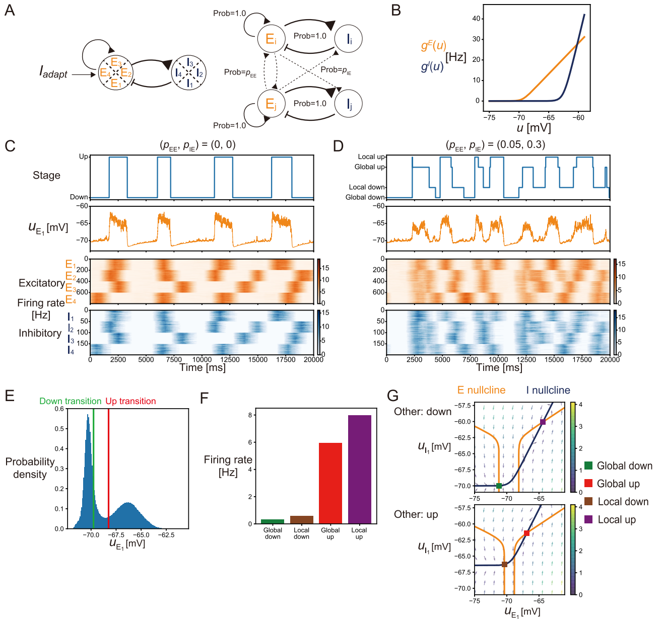
Fig. 3. The cortical network model exhibiting global and local slow waves. (A) The schematic description of the model. (Left) Model composed of four local networks. Each local network included 200 excitatory and 50 inhibitory neurons. (Right) Within a network, connections existed between two excitatory neurons, and between excitatory and inhibitory neurons, while two inhibitory neurons had no connections between them. Between different networks, there were sparse connections from excitatory to excitatory or inhibitory neurons but none from the inhibitory neurons. (B) The activation functions of excitatory and inhibitory neurons. Both functions were softplus functions, but the threshold and slope were greater for inhibitory neurons than those for the excitatory neurons. (C) The dynamics of the slow-wave model in the case of no connections between different local networks. The up and down states of the E1 population were classified using the mean membrane potential u_{E1} . The four networks independently transitioned between the up and down states. (D) The dynamics of the slow-wave model in the case that there exist sparse connections between different networks. The up and down states of the E1 population were classified into the global or local states depending on the states of the other populations. (E) The probability density of the membrane potential. The transition thresholds to the up and down states are indicated by red and green lines, respectively. (F) The mean firing rates of the E1 population in global down, local down, global up, and local up states. (G) The phase plane of the E1 and I1 population in the case that other populations are in down states (upper) or in up states (lower) (see SI Appendix Methods for details). Excitatory and inhibitory nullclines are shown as orange and blue lines, respectively. The four steady points corresponding to global down, local down, global up, and local up states are shown; the up state of E1 population is global or local when the other populations are in the up or down states, respectively, while the down state of E1 population is global or local when the other populations are in the down or up states, respectively. The u_{E1} values of four steady points followed global down < local down < global up < local up in ascending order.
