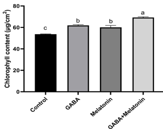
Figure 5. Effect of gamma-aminobutyric acid (GABA (20 \mu M)), melatonin (200 \mu M), and GABA (20 \mu M) + melatonin (200 \mu M) on chlorophyll content of Vicia faba . Different letters denote significant differences among different treatments. Means followed by the same letter are not significantly different at 5% probability level by LSD test.
