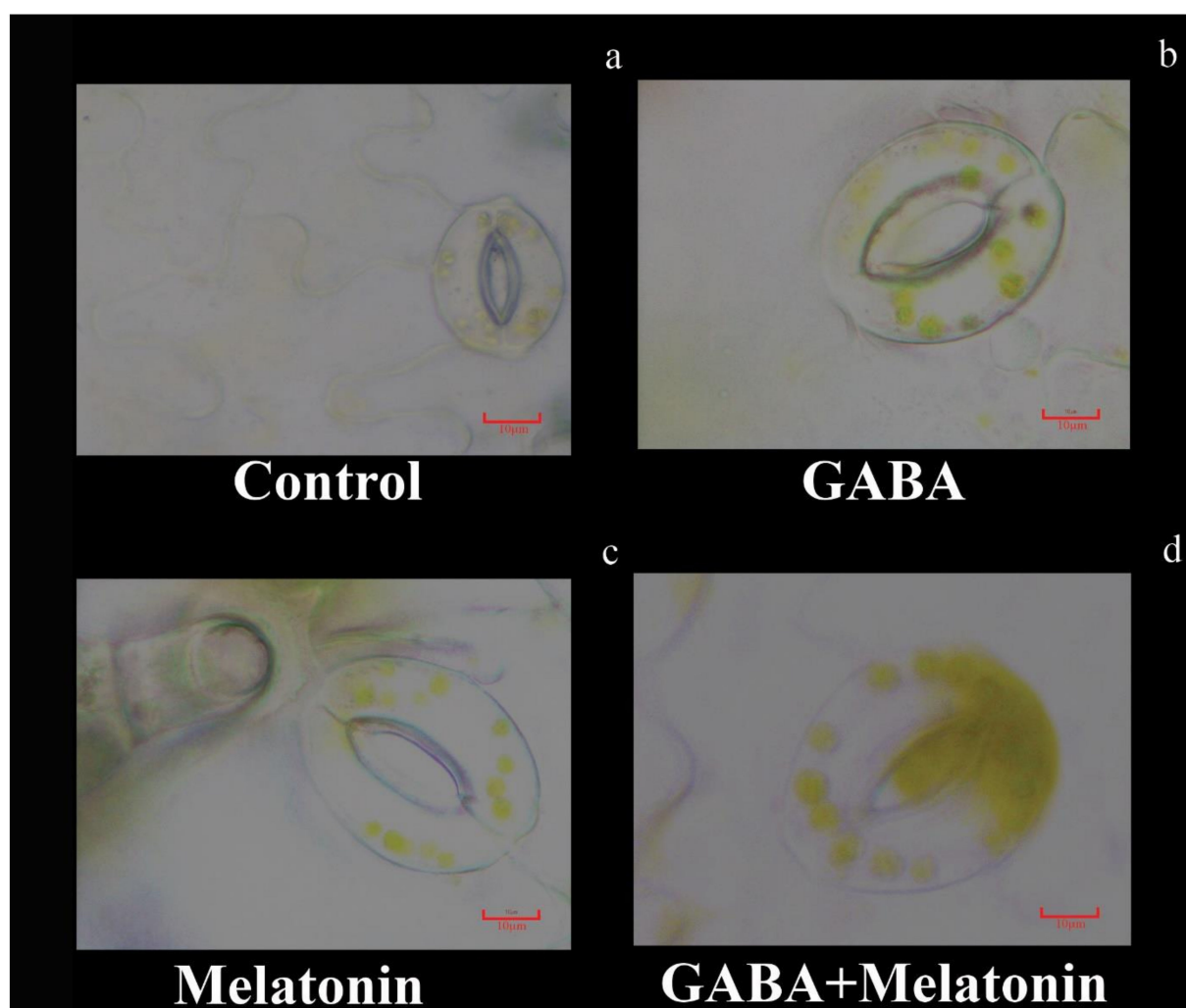
Figure 4. Effect of gamma-aminobutyric acid (GABA (20 \mu M)), melatonin (200 \mu M), and GABA (20 \mu M) + melatonin (200 \mu M) on stomatal characteristics of Vicia faba . Bar: (a–d): 10 \mu m.
