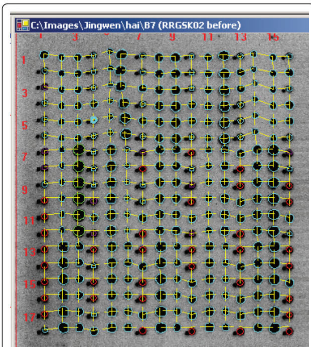
Figure 7 Actual Boundary and Flexible Grid Algorithms. Image and spot shifts among arrays are the major challenge for the automation of array image processing. The fixed spot grid cannot be applied to all images. The actual boundary and flexible grid algorithms are designed to make spot position and grid flexible enough to compensate the shifts. These algorithms are essential for the successful automation of array image analysis using MicroVigene™.
