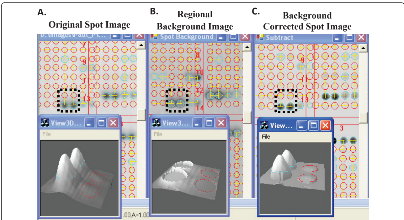
Figure 8 Regional Background Correction Algorithm. This algorithm is to correct the original spot signal intensity (A) with local background (B). The real spot signals (C) can be extracted. Four spots within the black dashed square boxes in 2D view are shown in the 3D view windows below. This algorithm improves accuracy, consistency, and sensitivity for image processed using MicroVigene™.
