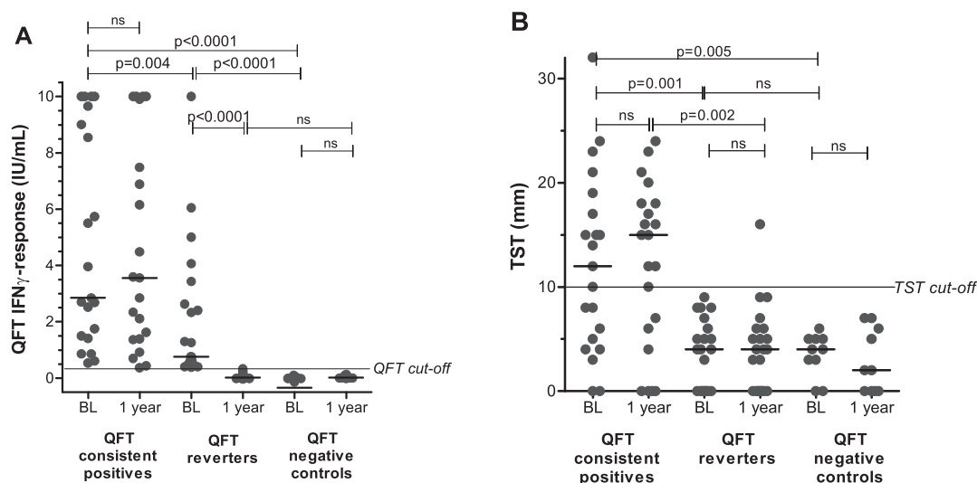
Figure 1. QuantiFERON Gold In-Tube (QFT) and Tuberculin Skin Test (TST) responses. (A) The magnitude of the QFT response and (B) the TST response in QFT consistent positives ( n = 21 ), QFT reverters ( n = 21 ) and QFT negative controls ( n = 10 ) at baseline (BL) and after 1 year. Unpaired and paired analyses was performed with Mann-Whitney U test and Wilcoxon Signed rank test where appropriate. Horizontal lines represent median values.
