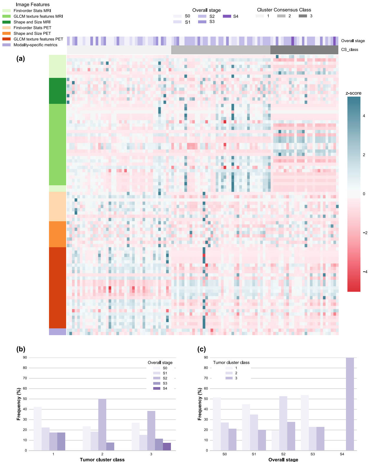
Fig. 2 PET and MR radiomics vs. tumor overall stage heatmap. a A heatmap of the PET and MR radiomic features is shown with the corresponding tumor overall stage and the tumor clusters resulted from the optimized consensus clustering. b The proportion of different tumor overall stages is shown for each tumor cluster category. The frequency is shown with respect to the total number of tumors in each tumor cluster category. c The proportion of different tumor clusters is shown for each tumor overall stage category. The frequency is shown with respect to the total number of tumors in each tumor overall stage category
