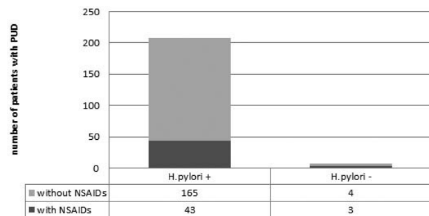
Fig. 1: Frequency of PUD and Helicobacter pylori status. Of the 215 patients who were found to have PUD 96.7% were H.pylori positive and only 4 patients (1.8%) were negative for both H.pylori and NSAIDs.
