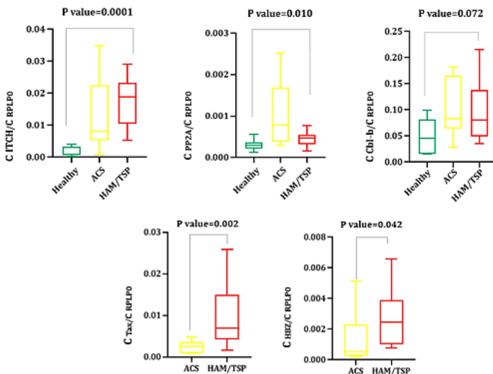
Fig. 1. The cellular and viral gene expression levels; ITCH E3 ligase (A), Protein phosphatase 2 A, PP2A, (B), Cbl-b E3 ligase (C), Tax (D), and HBZ (E) in the three sample groups; healthy individuals, ACs, and HAM/TSP.
